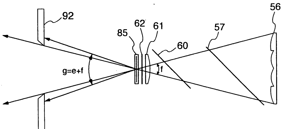
FIG. 12 PRIOR ART
