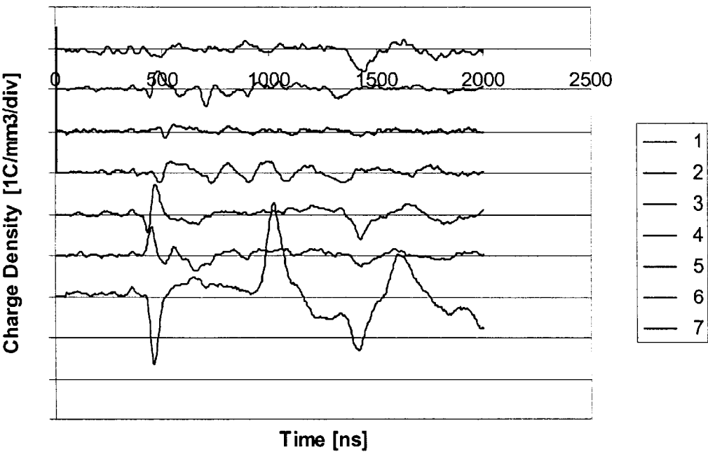
Figure 2. Space Charge Measurement after 24 hours at - 20 kV/mm
