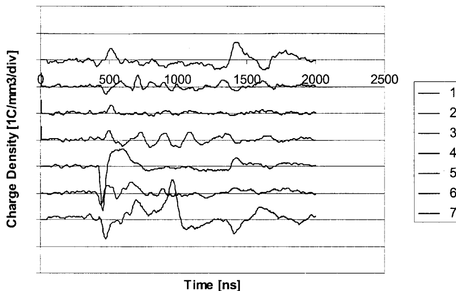
Space Charge Measurement after 24 hours at + 20 kV/mm
