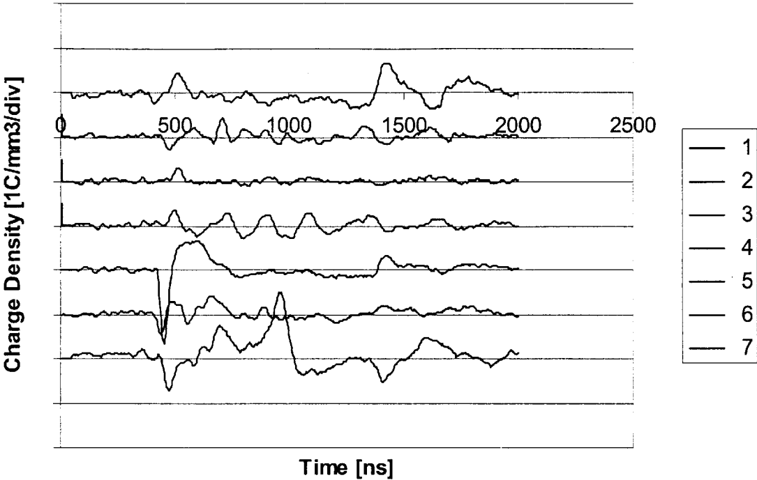
Figure 1. Space Charge Measurement after 24 hours at + 20 kV/mm
