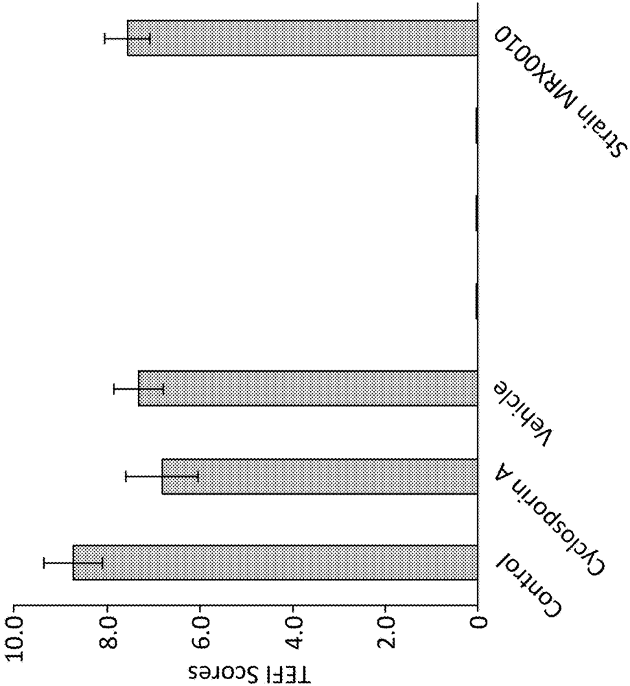
FIG. 3 TEFI Scores
