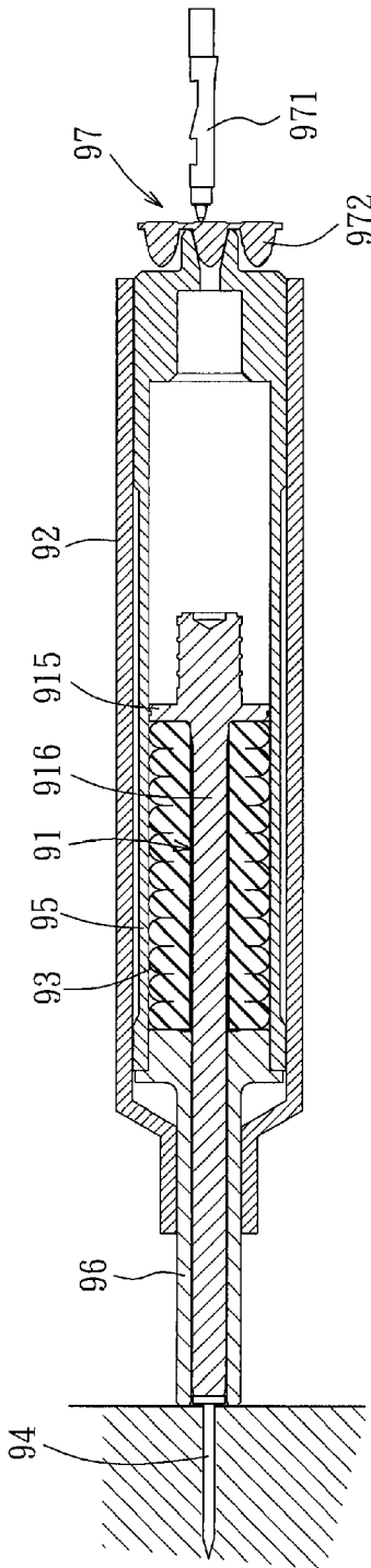
FIG. 2 PRIOR ART
