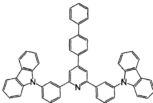
Compound C1
