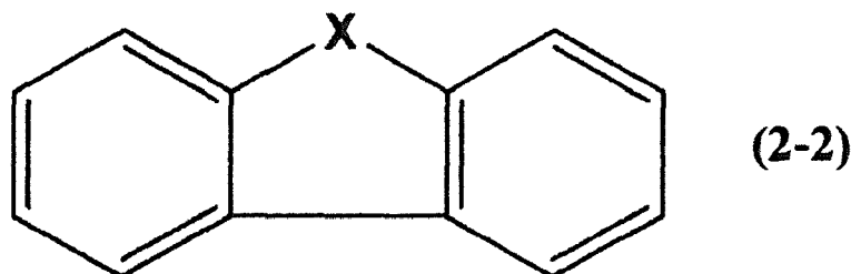
[Chem. 16]
