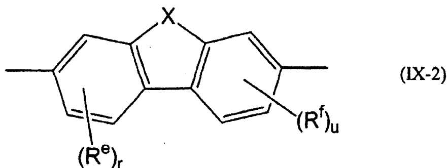
[Chem. 42]
