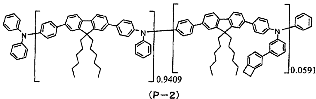
[Chem. 52]
