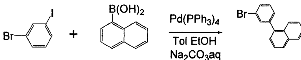
Compound 5
