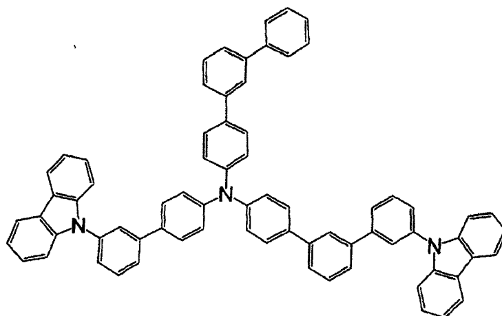
[Chem. 54]
