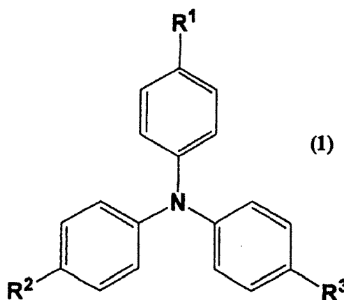
[Chem. 1]
