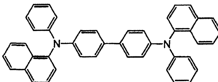
[Chem. 1]
