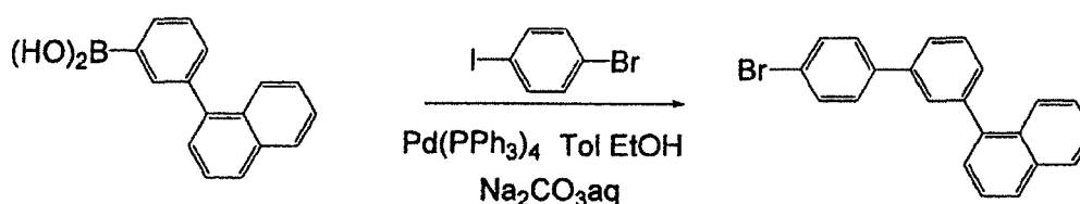
Compound 6
