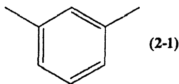
[Chem. 2]
