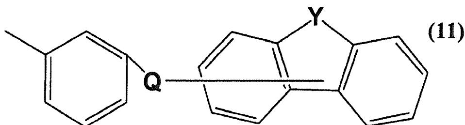
[Chem. 10]
