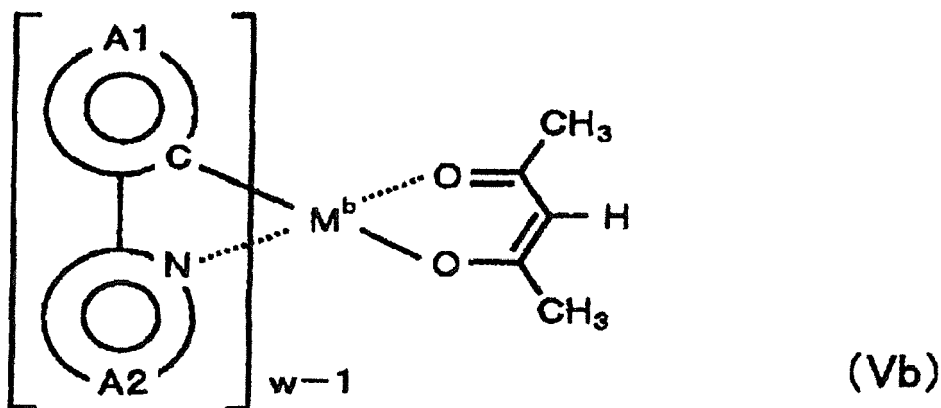
[Chem. 33]
