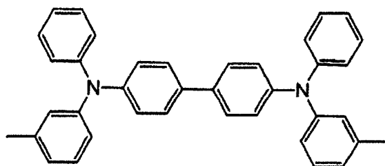
[Chem. 4]
