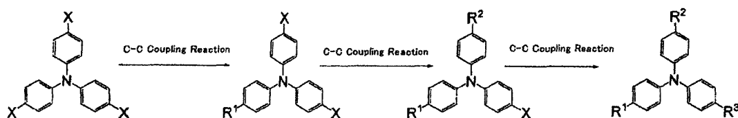
[Chem. 27]
