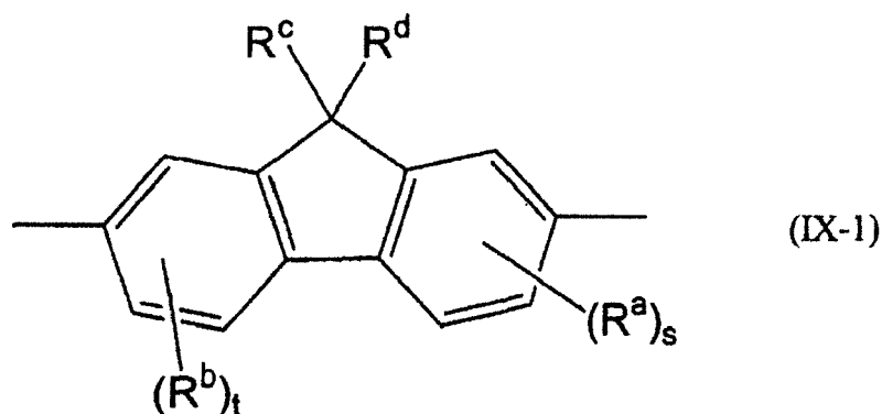
[Chem. 41]
