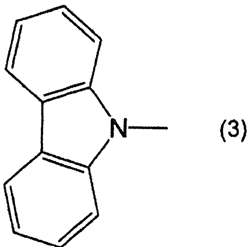
[Chem. 4]
