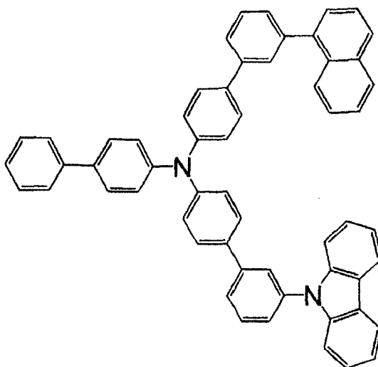
Compound III
