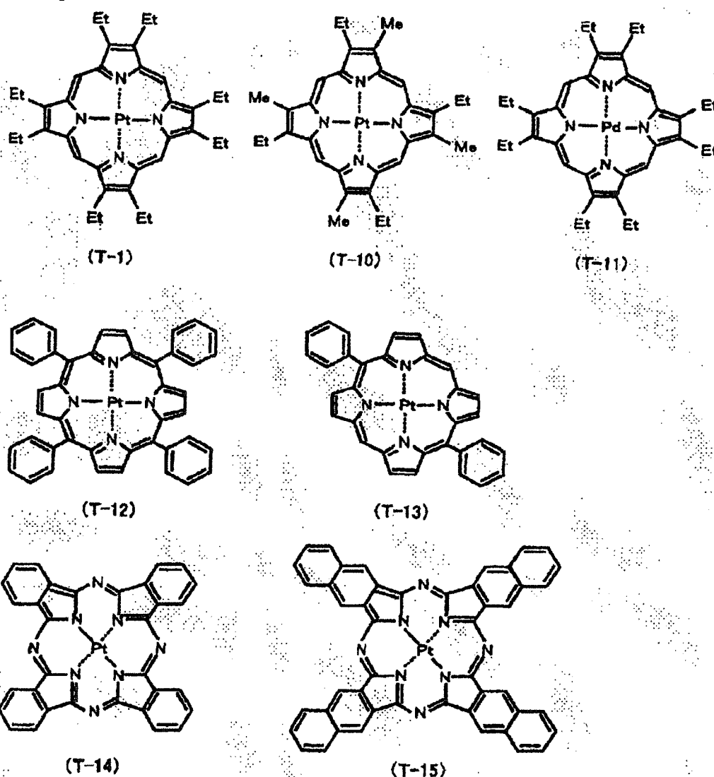
[Chem. 37]
