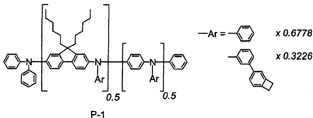
[Chem. 51]
