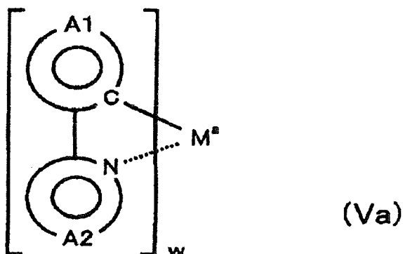
[Chem. 32]
