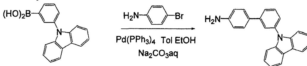
Compound 8
