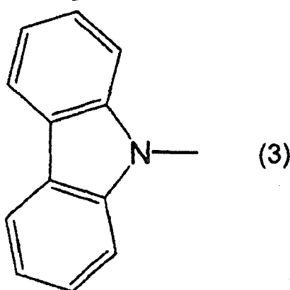
[Chem. 17]
