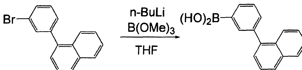
Compound 5
