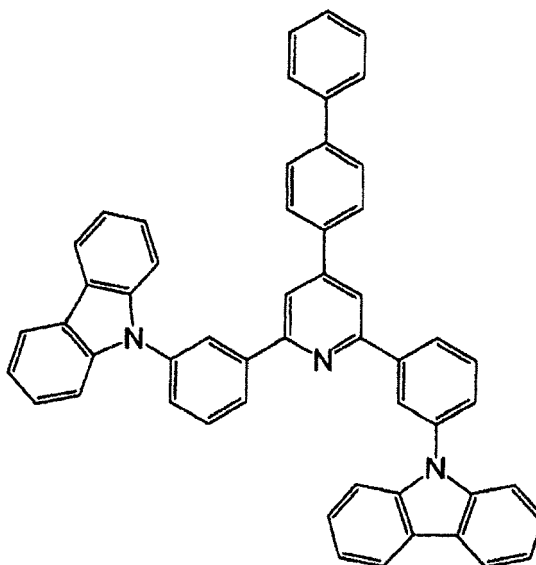
Compound C2
