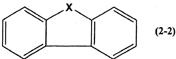
[Chem. 8]
