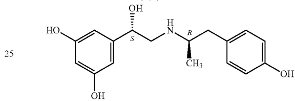
(S,R)-Fenoterol
