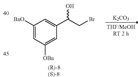
Scheme I
