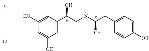
(R,R)-Fenoterol
