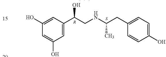
(R,S)-Fenoterol
