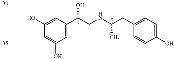
(S,S)-Fenoterol
