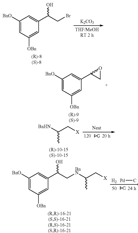
Scheme I: An exemplary synthesis of 4 stereoisomers of 1-6 including the coupling of the epoxide formed from either (R)- or (S)-3',5'-dibenzyloxyphenylbromohydrin with the (R)- or (S)-enantiomer of the appropriate benzyl-protected 2-amino-3-benzylpropane (1-5) or the (R) or (S)-enantiomer of N-benzyl-2-aminoheptane (6).
