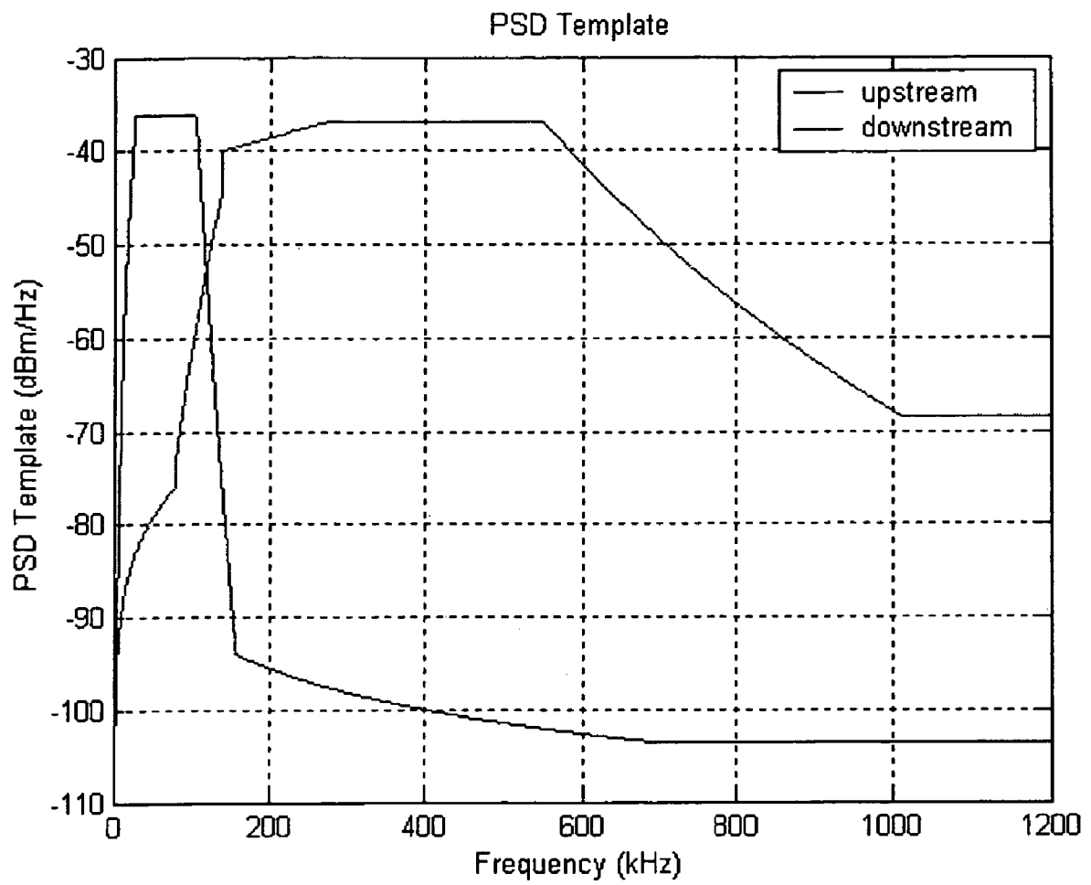
Figure 2: U2 and D2 PSD Templates, average values.
