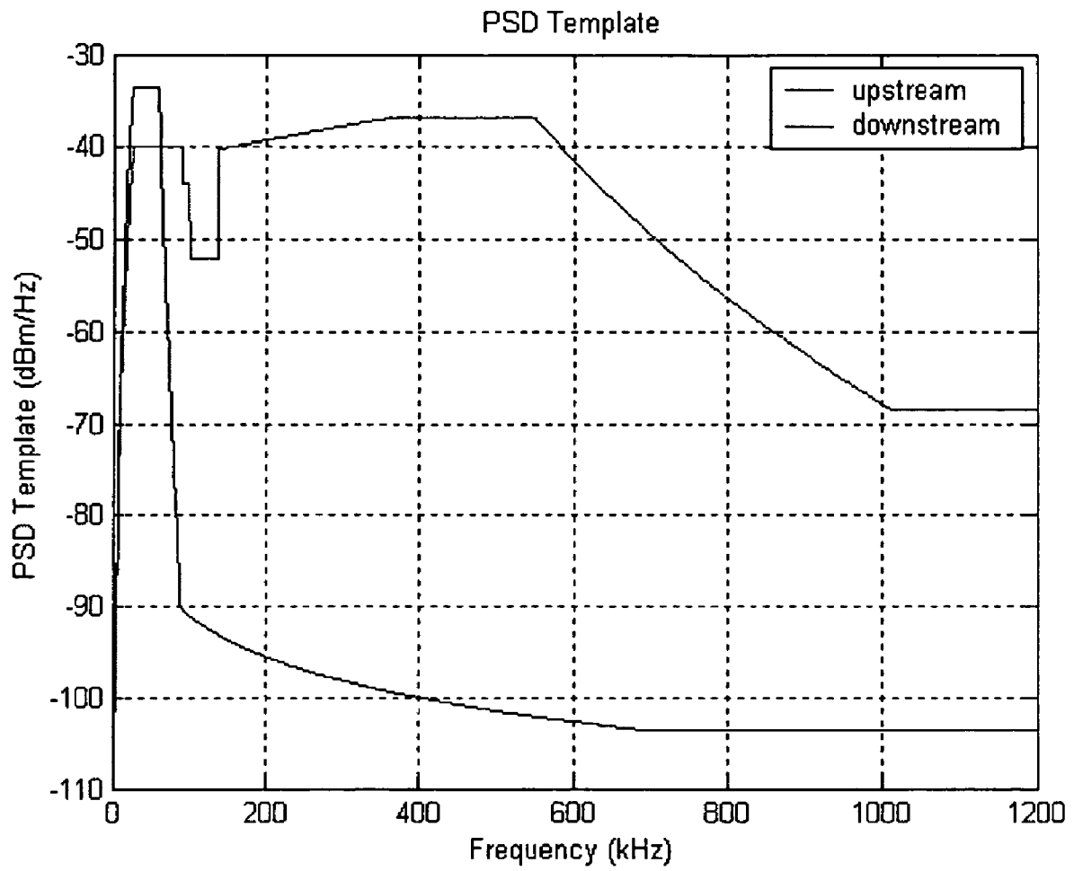
Figure 1: U1 and D1 PSD Nominal Templates.
