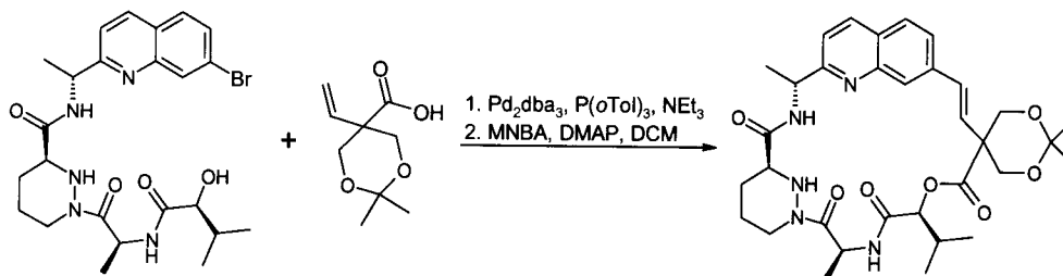
Compound 113.
