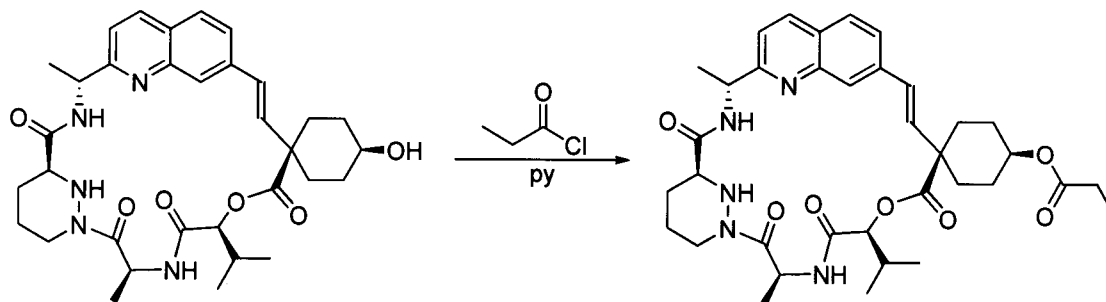
Compound 111
