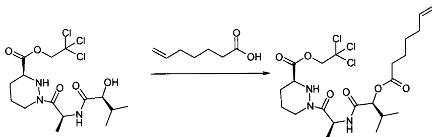
Compound 8a
