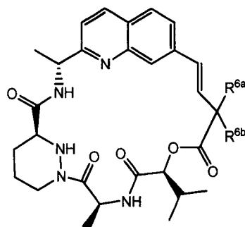
Formula II-c
