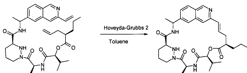
Compound 4
