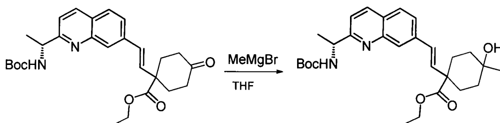
Compound 89b
