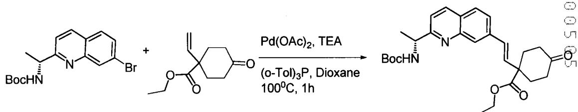
Compound 89a
