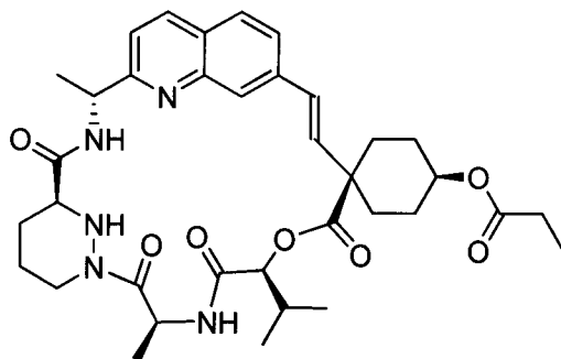
Compound 111
