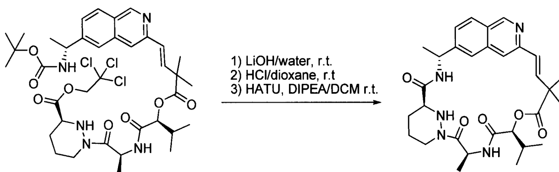
Compound 69
