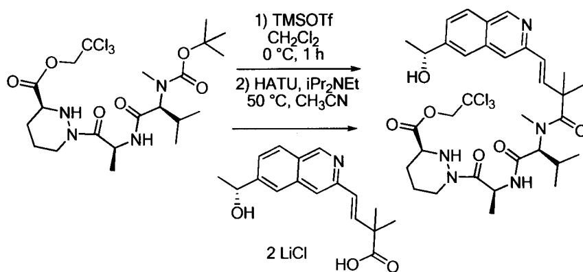
Compound 22g
