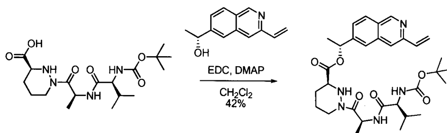
Compound 20e
