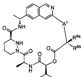
Formula (II-a)
