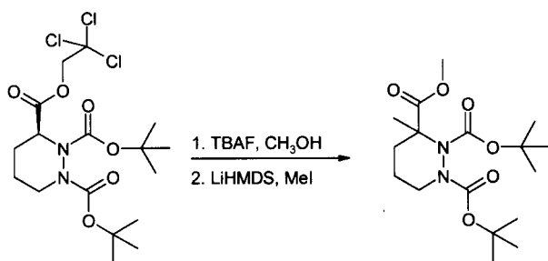
Compound 94a. 3-Methyl-tetrahydro-pyridazine-1,2,3-tricarboxylic acid 1,2-di- tert -butyl ester 3-methyl ester
