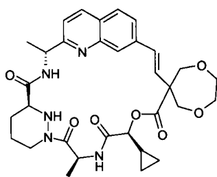
Compound 93a. (S)-4-Benzyl-3-(2-cyclopropyl-acetyl)-oxazolidin-2-one
