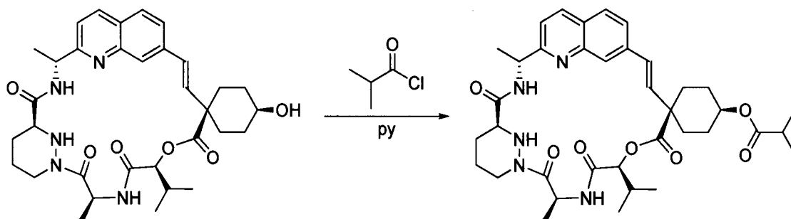
Compound 81
