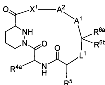
Formula III
