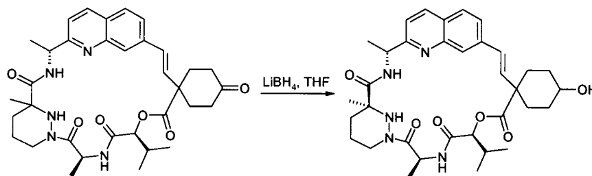
Compound 94.
