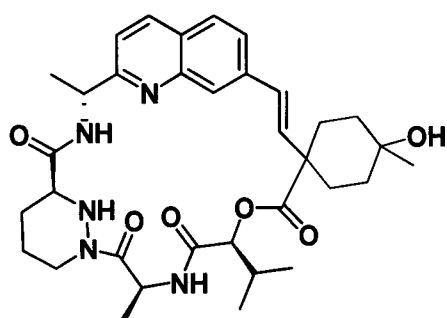
Compound 89a
