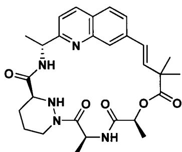
Compound 61a
