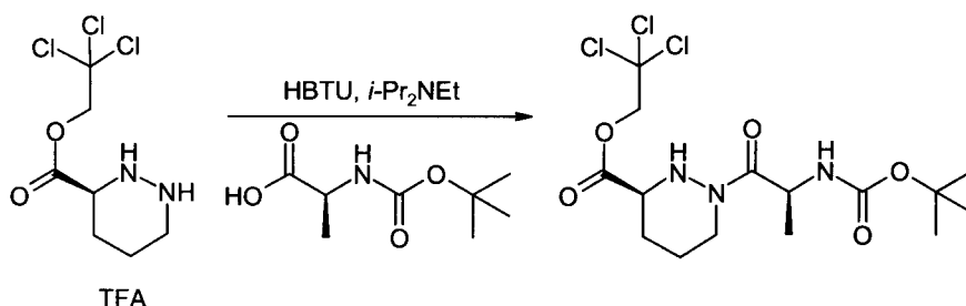
Compound 1d
