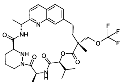
Compound 56a. (R)-2-Methyl-2-trifluoromethoxymethyl-but-3-enoic acid
