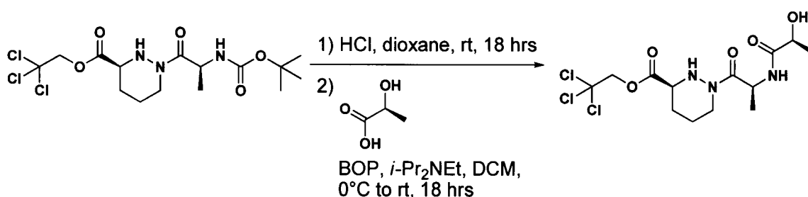
Compound 61a
