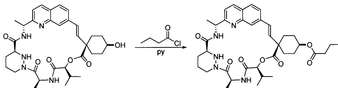
5 Compound 82
