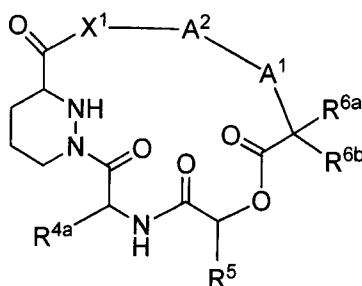
Formula II
