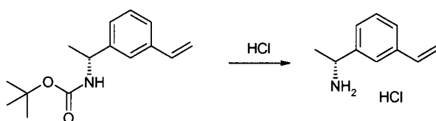
Compound 1j
