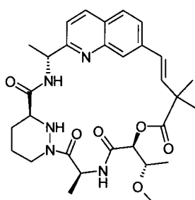
Compound 54a. (2S,3S)-2-Hydroxy-3-methoxy-butyrac acid
