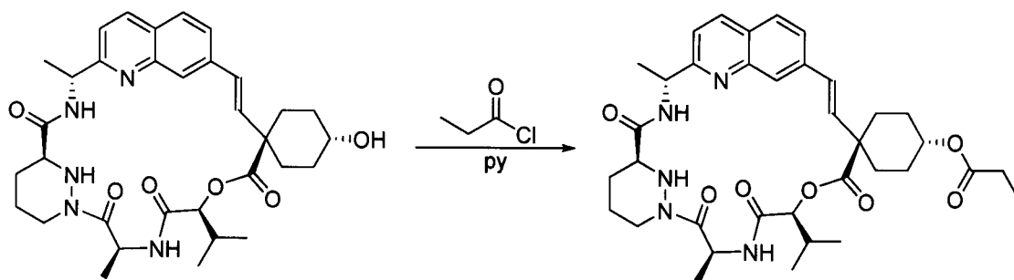
Compound 109
