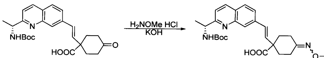
Compound 83b
