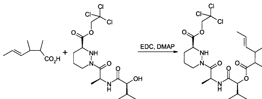
Compound 11c
