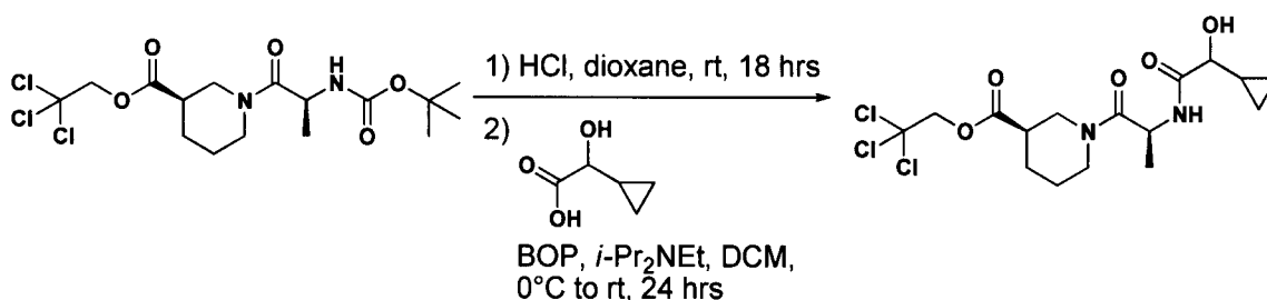
Compound 66a
