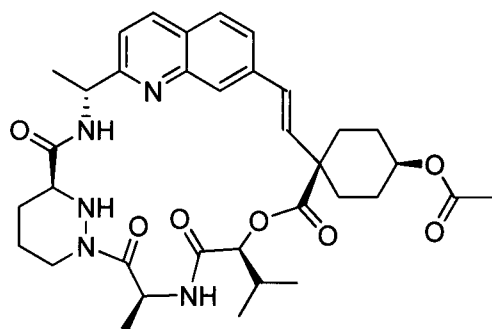
Compound 112
