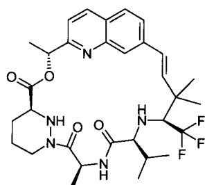
Compound 31a: (S)-3-Methyl-2-[2,2,2-trifluoro-ethylideneamino]-butyric acid methyl ester
