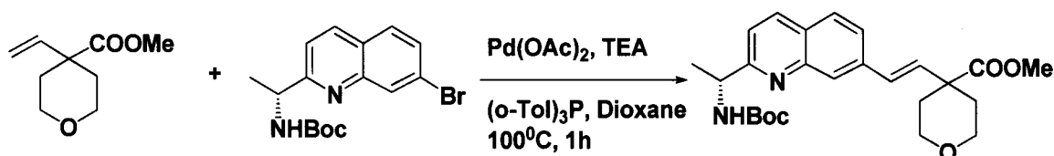
Compound 88d
