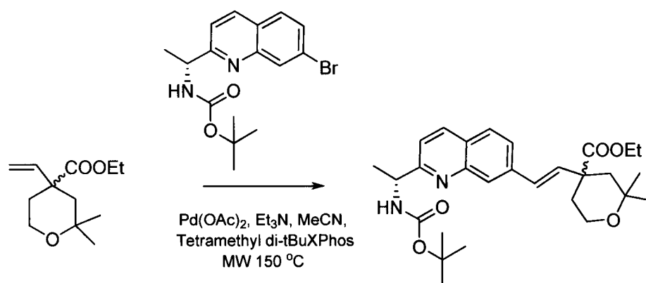
Compound 90a
