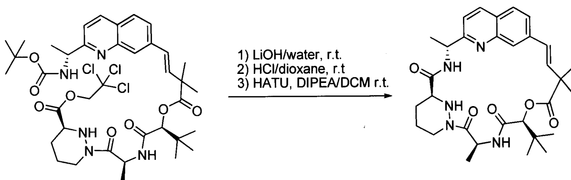
Compound 70
