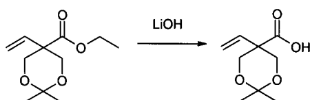
Compound 113a. 2,2-Dimethyl-5-vinyl-[1,3]dioxane-5-carboxylic acid
