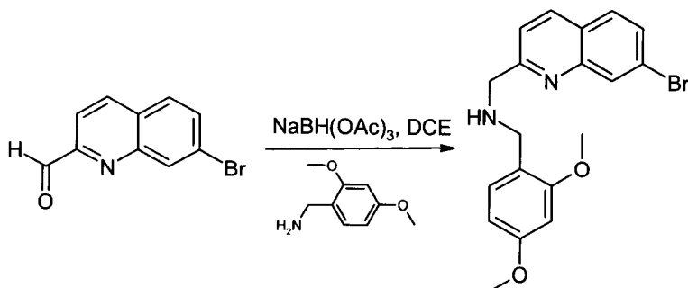
Compound 37a. (7-Bromo-quinolin-2-ylmethyl)-(2,4-dimethoxy-benzyl)-amine
