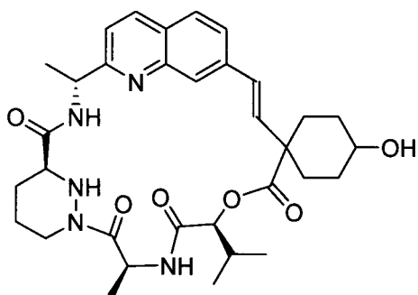
Compounds 74 and 75
