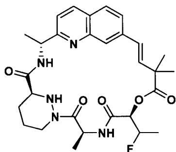
Compound 68a
