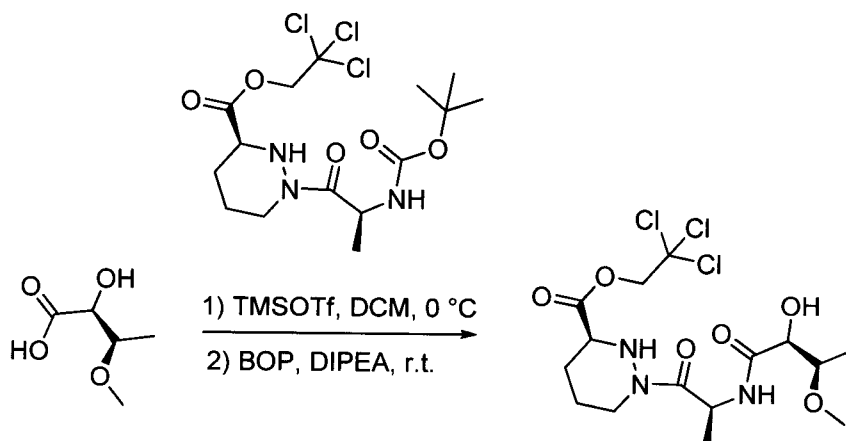
Compound 60b:
