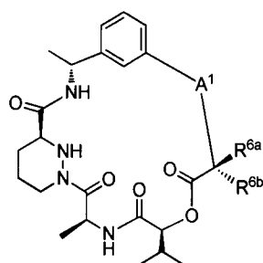
Formula (II-b)
