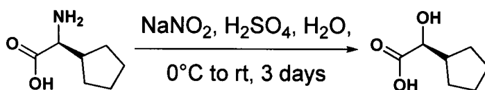
Compound 63a
