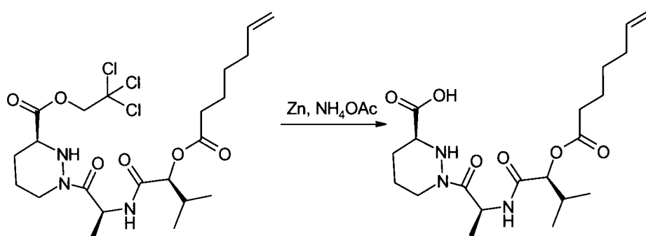
Compound 8b
