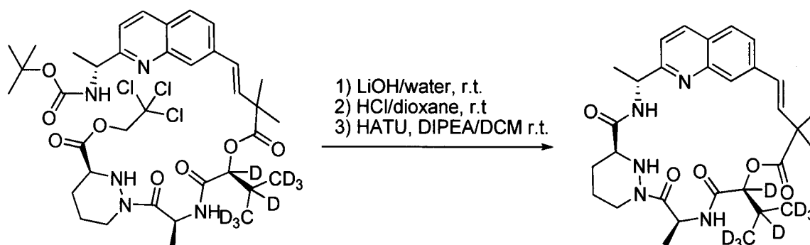
Compound 59.
