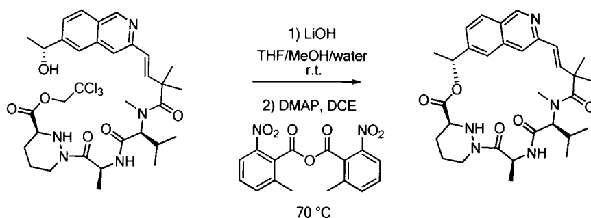
Compound 22
