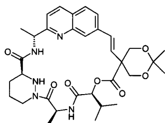
Compound 113a. 2,2-Dimethyl-5-vinyl-[1,3]dioxane-5-carboxylic acid
