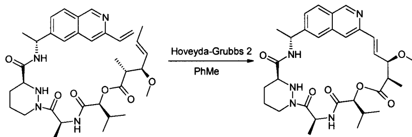
Compound 2
