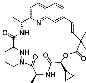
Compound 78a
