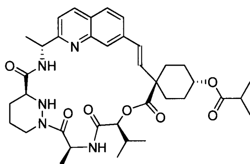
Compound 80
