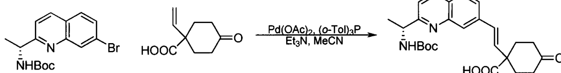
Compound 83a
