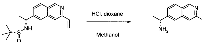
Compound 2j
