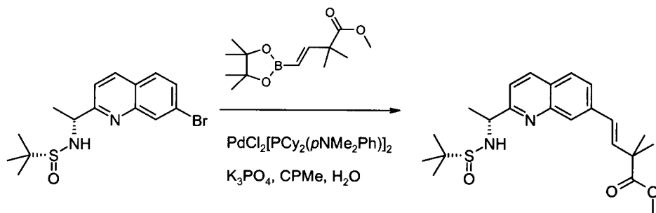
18d
