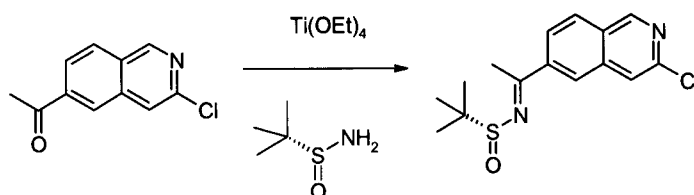
Compound 2g
