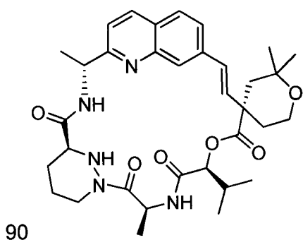
Compound 90a
