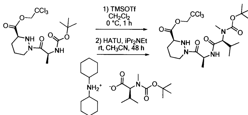
Compound 22a
