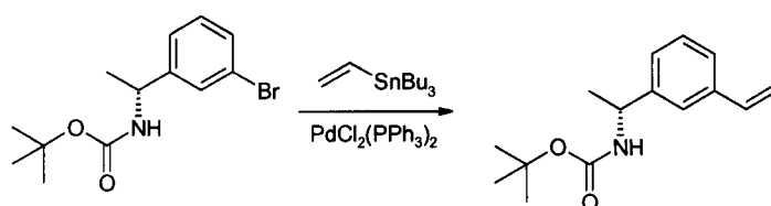
Compound 1i
