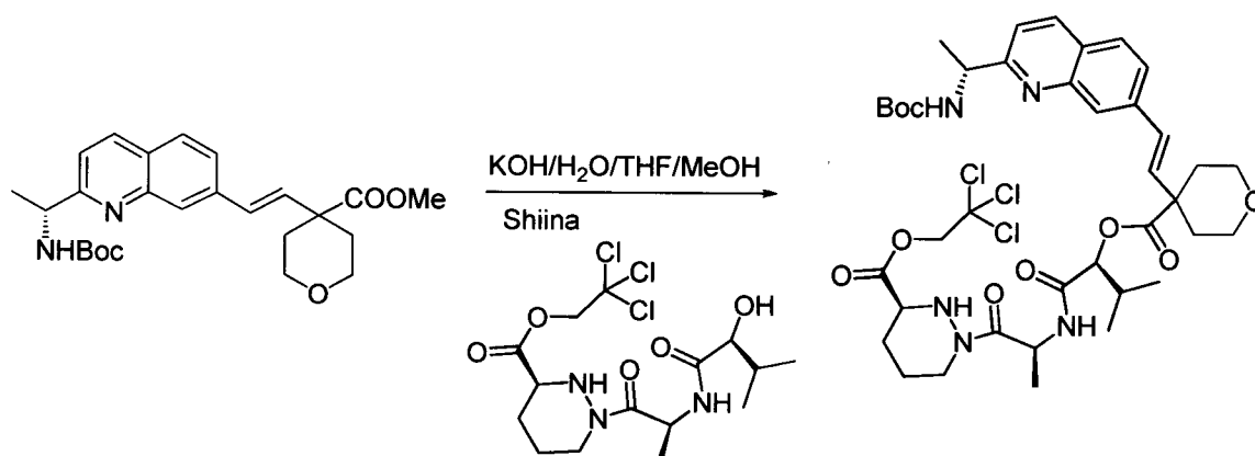
Compound 88e
