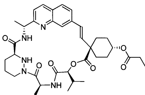
Compound 109
