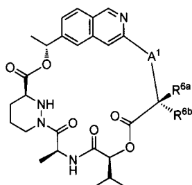
Formula (II-a2)
