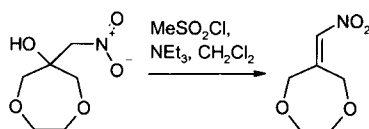
Compound 57b. 6-Nitromethylene-[1,4]dioxepane
