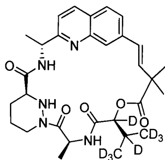
Compound 59a:
