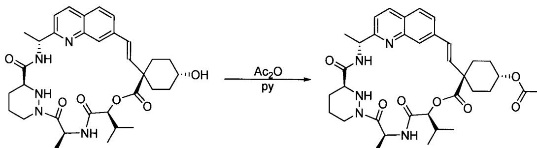
Compound 110
