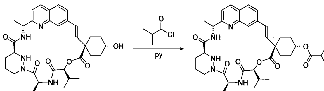
Compound 80
