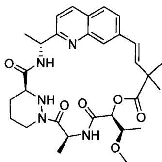
Compound 60a:
