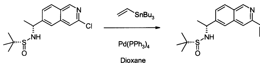
Compound 2i
