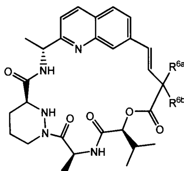
Formula II-c
