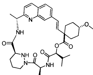
Compound 92a
