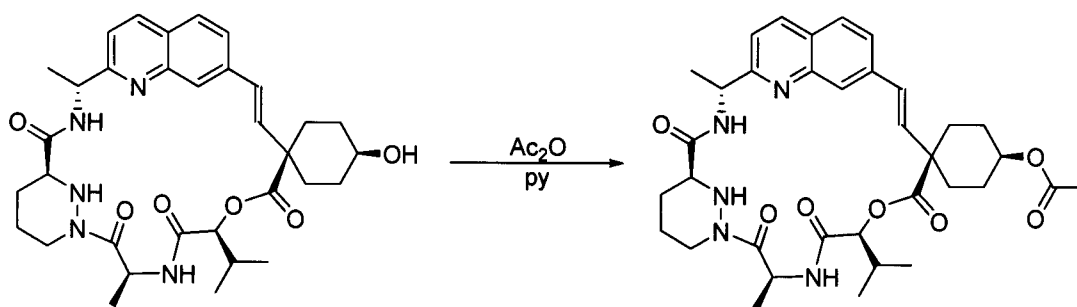
Compound 112
