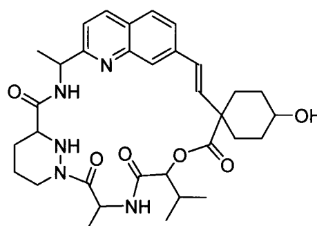
Compounds 76 and 77
