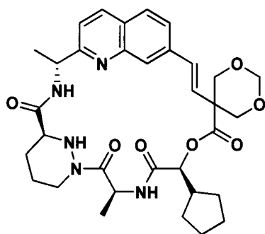
Compound 63a
