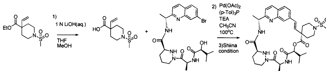
Compound 85
