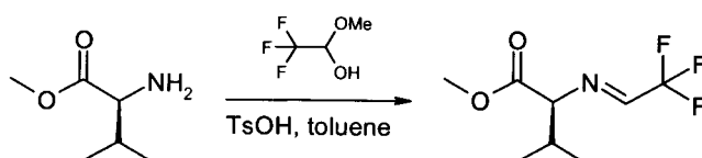
Compound 31a: (S)-3-Methyl-2-[2,2,2-trifluoro-ethylideneamino]-butyric acid methyl ester
