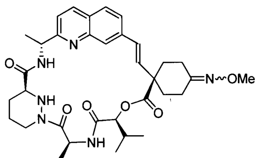
Compound 83a
