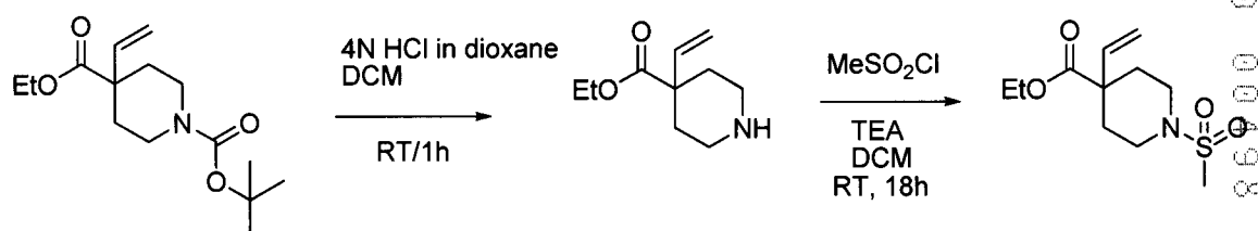
Compound 85a
