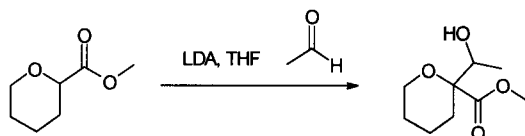
Compound 49a. 2-(1-Hydroxy-ethyl)-tetrahydro-pyran-2-carboxylic acid methyl ester
