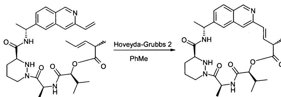
Compound 5
