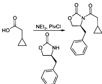
Compound 93a. (S)-4-Benzyl-3-(2-cyclopropyl-acetyl)-oxazolidin-2-one
