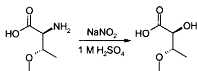
Compound 54a. (2S,3S)-2-Hydroxy-3-methoxy-butyrac acid
