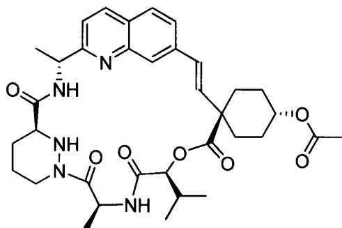
Compound 110
