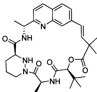
10 Compound 70a:
