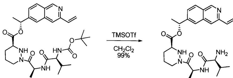
Compound 20f
