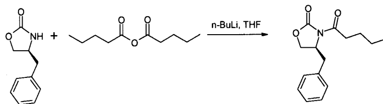
Compound 4a
