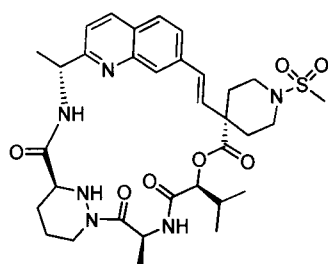
Compound 85a
