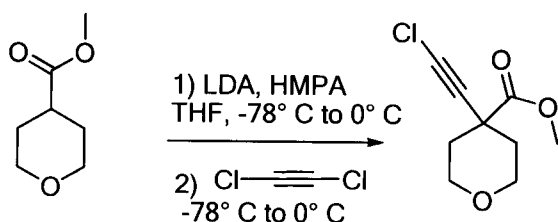
Compound 88b: 4-Chloroethynyl-tetrahydro-pyran-4-carboxylic acid methyl ester
