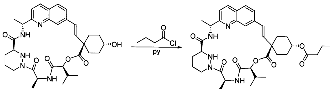
Compound 108
