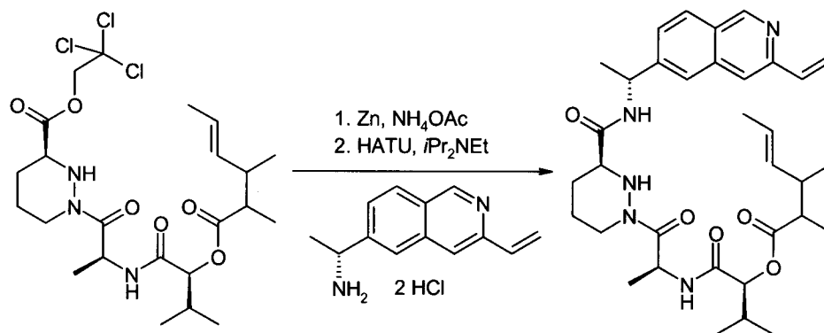
11d
