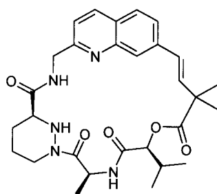
Compound 37a. (7-Bromo-quinolin-2-ylmethyl)-(2,4-dimethoxy-benzyl)-amine
