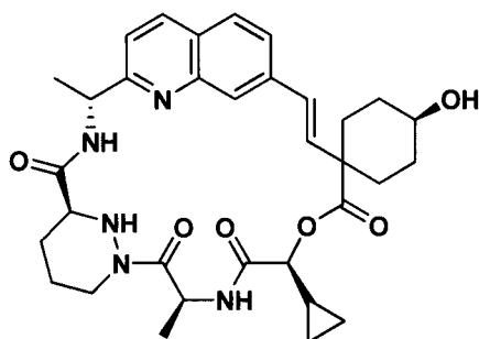
Compound 66a
