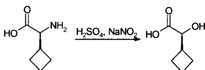
Compound 52a. (S)-Cyclobutyl-hydroxy-acetic acid
