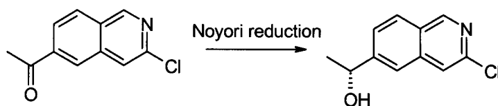
Compound 20a
