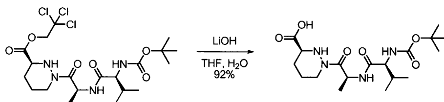
Compound 20d
