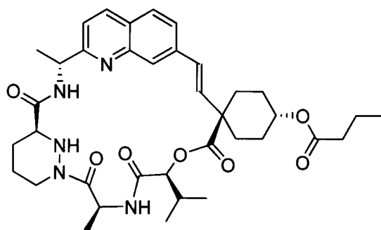
Compound 108
