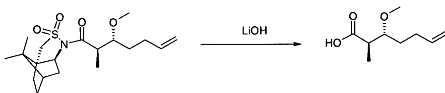
Compound 1c
