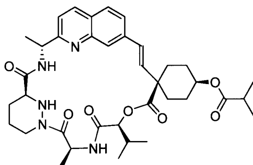
Compound 81
