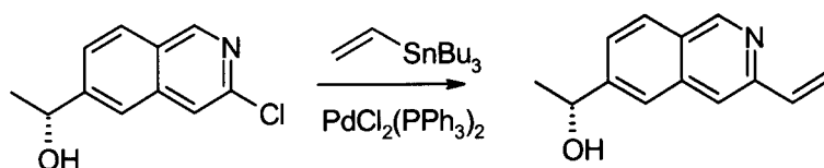
Compound 20b
