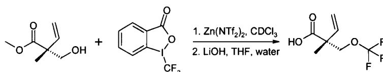
Compound 56a. (R)-2-Methyl-2-trifluoromethoxymethyl-but-3-enoic acid
