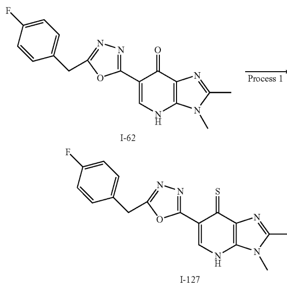
Compound I-127
