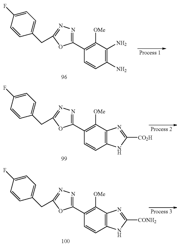
Compound I-133
