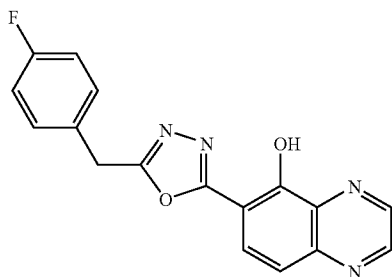
Compound I-132
