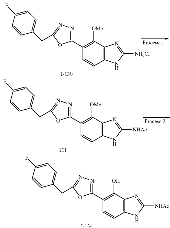
Compound I-134
