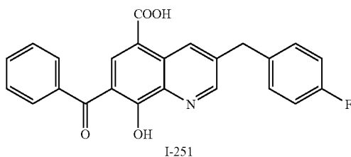
Compound I-251
