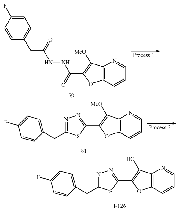
Compound I-126
