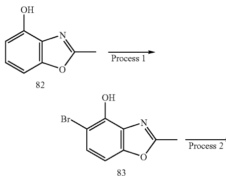
Compound I-128
