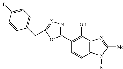
I-106 ~ I-121
