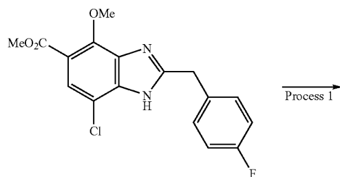
Compound I-32
