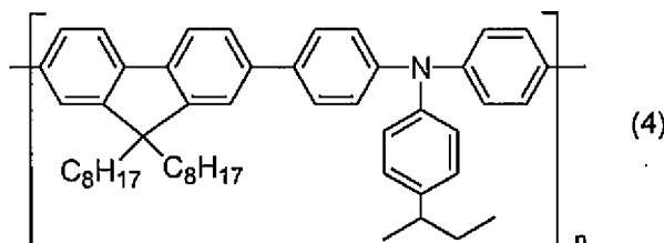
[Chemical formula 5]
