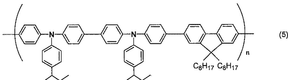
[Chemical formula 6]
