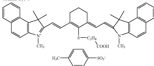
Cyanine Dye C
