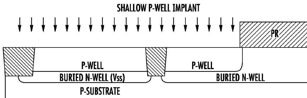
SRAM CELL PROCESS - BIPOLAR SELECT TRANSISTORS
