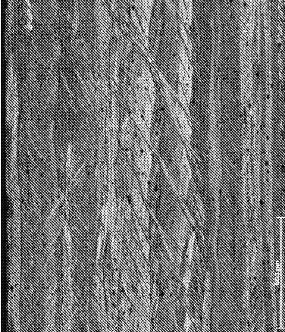
6xxx+Cu+Zn Aluminum Alloy – 60% CW
