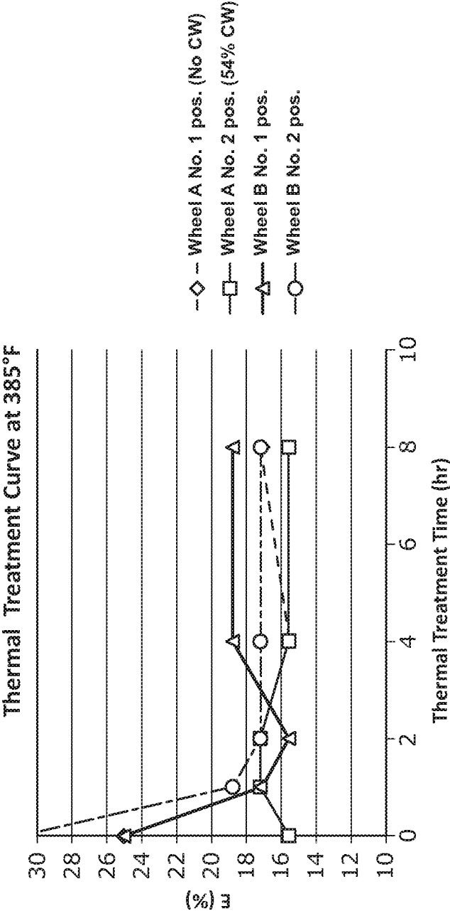
Elongation Thermal Treatment Curve at 385°F
