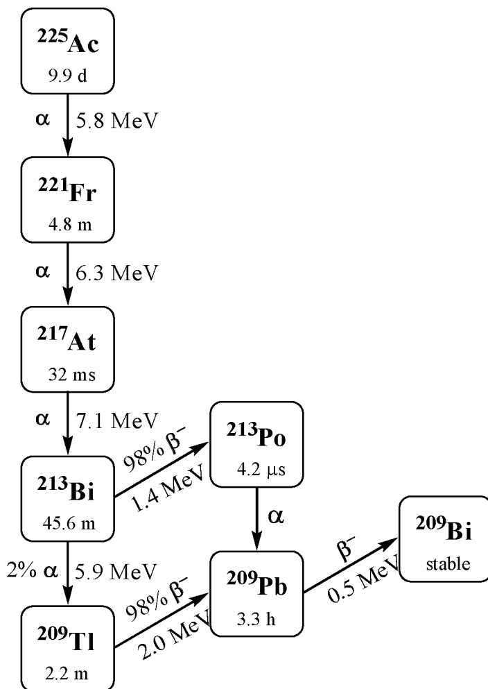
FIG. 1 (PRIOR ART)
