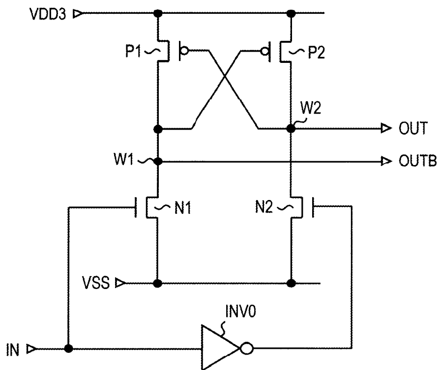
FIG. 11 PRIOR ART
