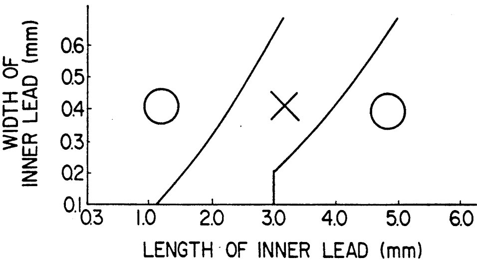
FIG. 21 (PRIOR ART)
