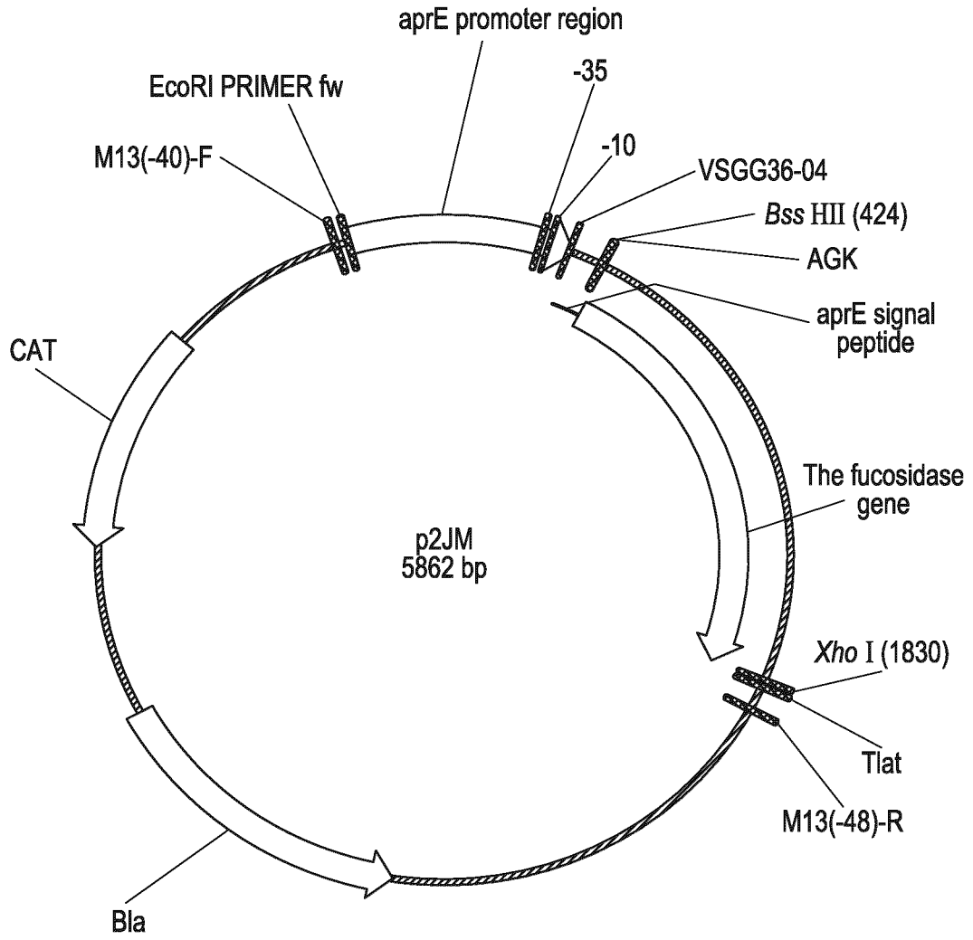
Exemplary plasmid map p2JM
