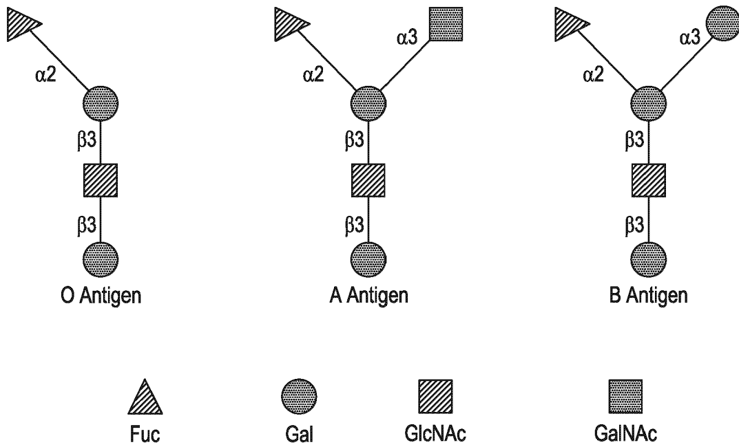
Structures of A, B, and O Oligosaccharide Antigens Abbreviations: Fuc=L-fucose; Gal=D-galactose; GalNAc = N-acetylgalactosamine; GlcNAc = N-acetylglucosamine
