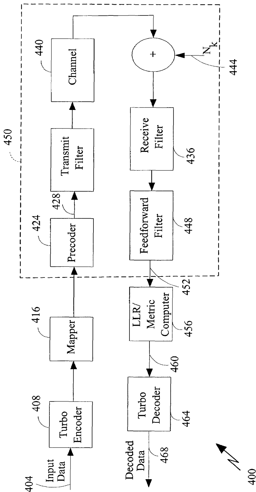
FIG. 4 COMMUNICATION SYSTEMS WITH TURBO CODE AND PRECODER
