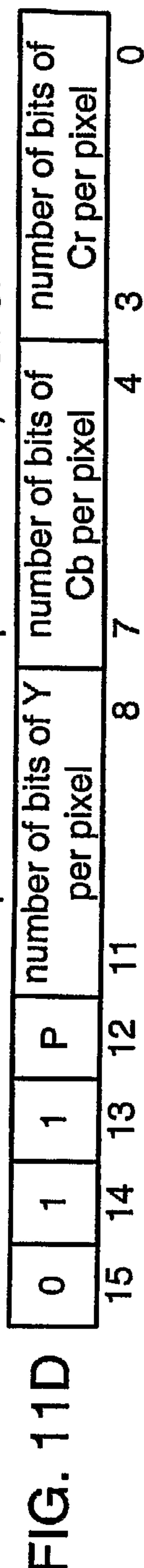
Video Data Format Descriptor - Color Component Video, Y Cb Cr
