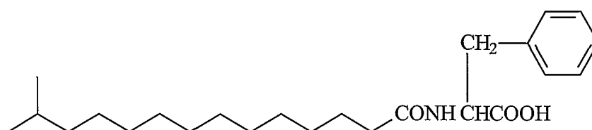
N-(13-Methyl-tetradecanoyl)-L-alanine
