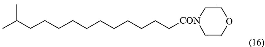
N-(13-Methyl-tetradecanoyl) morpholine
