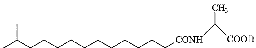
N-(13-Methyl-tetradecanoyl)glycine
