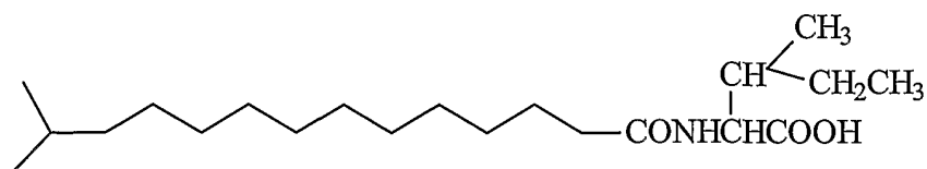
N-(13-Methyl-tetradecanoyl)-L-isoleucine
