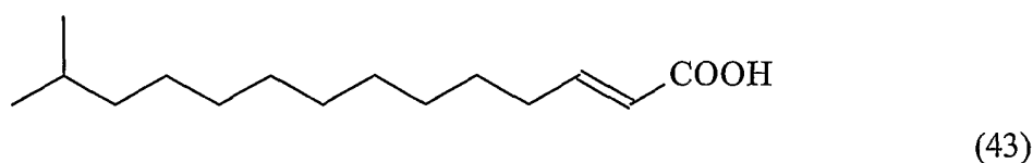
15-Methyl-2-hexadecenoic acid
