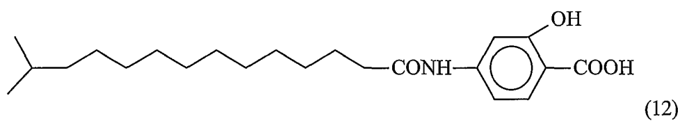
N-(3-Hydroxy-4-carboxylphenyl)-13-methyl-tetradecanamide
