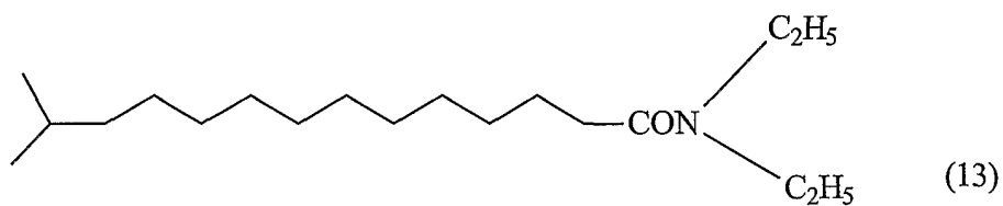
N,N-Diethyl-13-methyl-tetradecanamide
