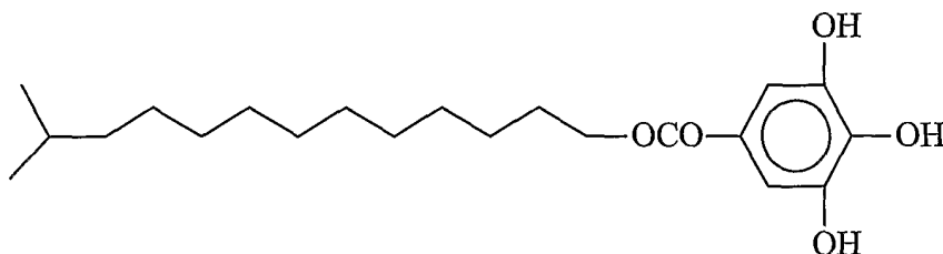
13-Methyltetradecyl-3,4,5-trihydroxy benzoate
