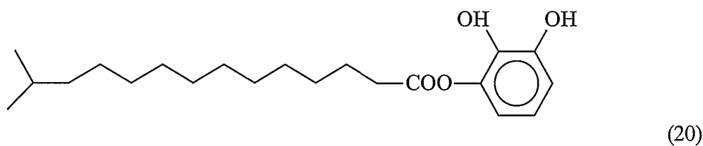
(2,3-Dihydroxy phenyl)-13-methyl-tetradecanate
