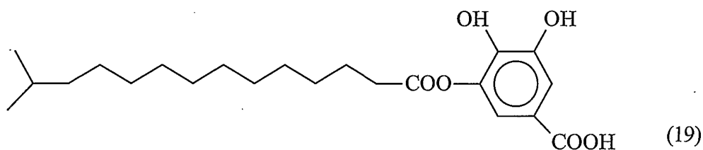
(5-Carboxy-2,3-dihydroxy phenyl)-13-methyl-tetradecanate
