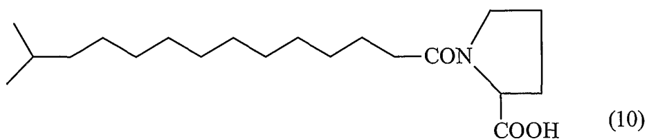
N-(13-Methyl-tetradecanoyl)-L-proline
