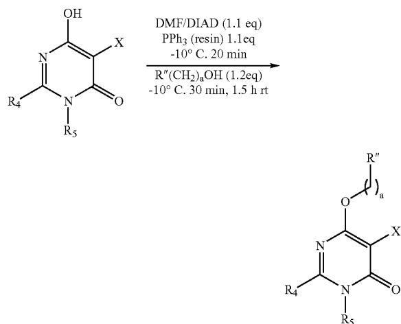
Scheme 10
