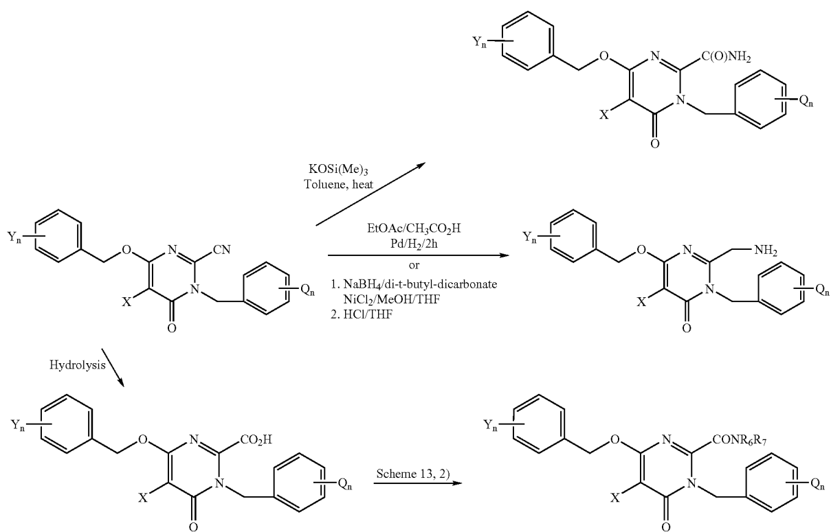
Scheme 9
