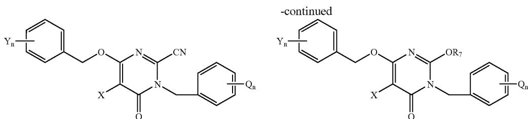
Scheme 8
