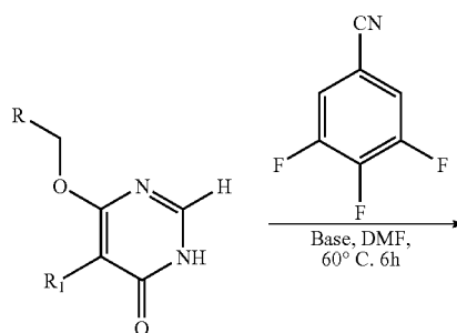
Scheme 12
