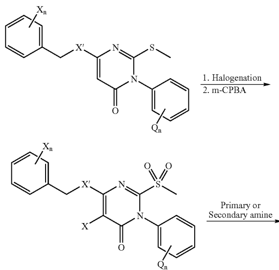
Scheme 24
