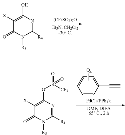
Scheme 11
