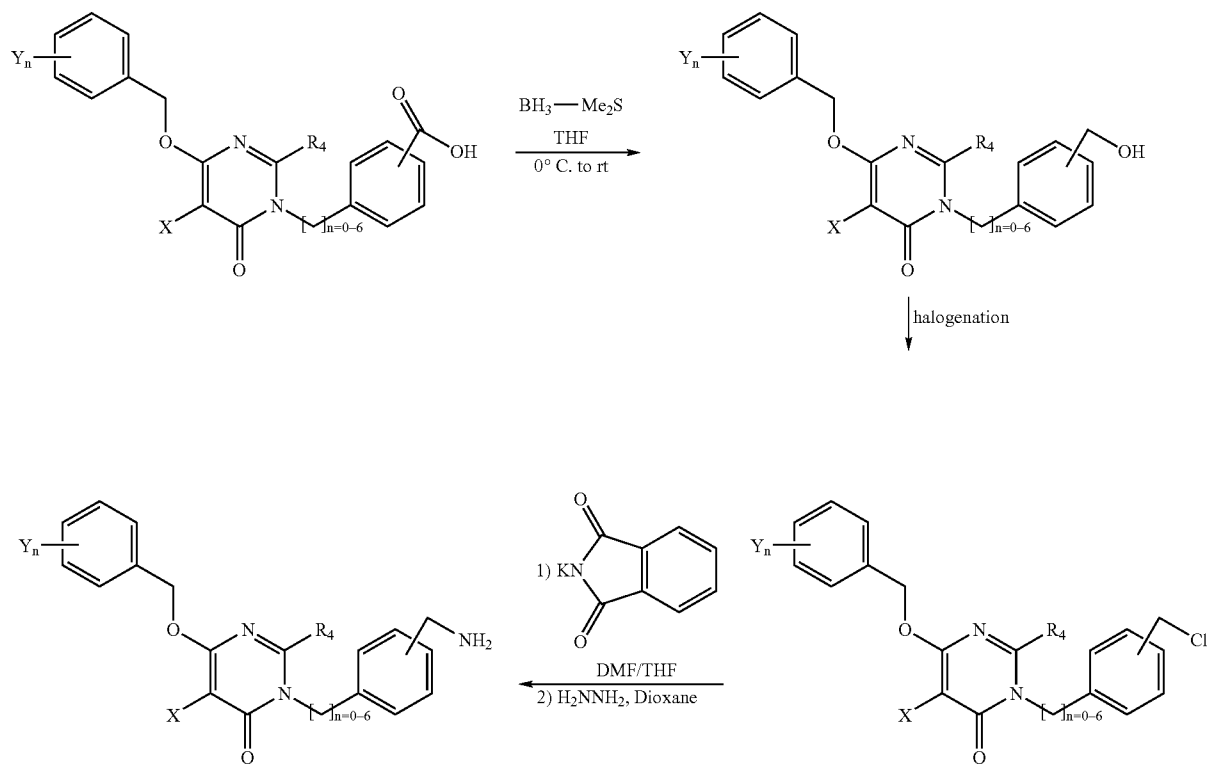
Scheme 14
