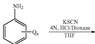
Scheme 23
