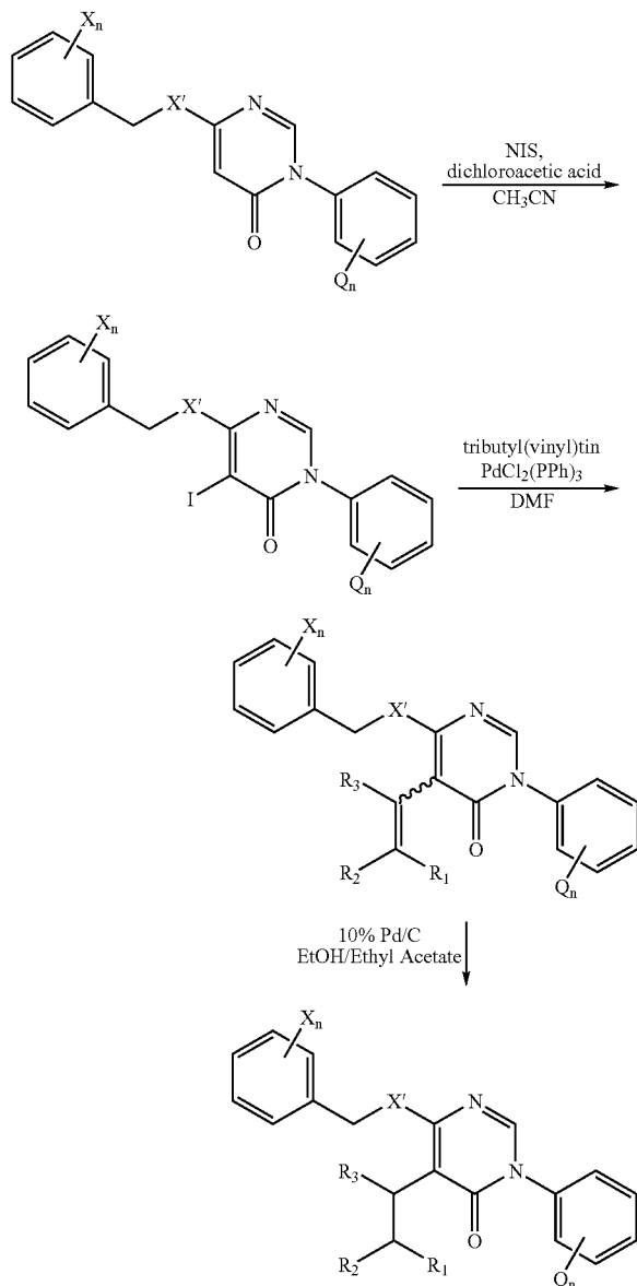
Scheme 25
