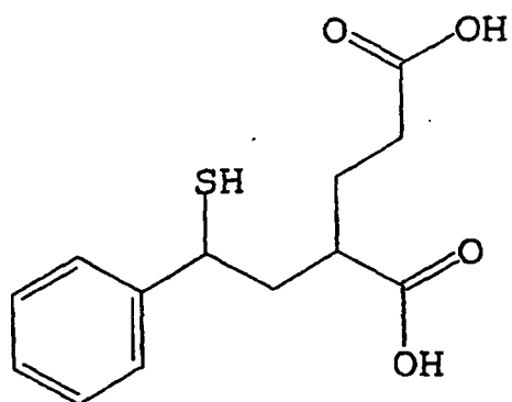
2-(2-phenyl-2-sulfanylethyl)pentanedioic acid
