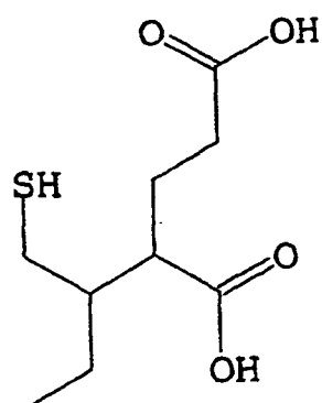
2-(1-ethyl-2-sulfanylethyl)pentanedioic acid
