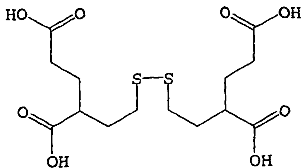
2-[2-[(3,5-dicarboxypentyl)dithio]ethyl]pentanedioic acid
