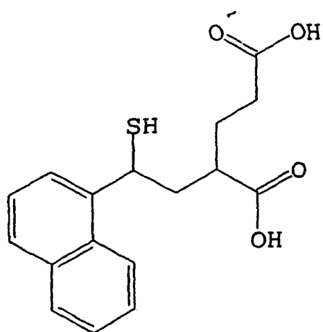
2-(2-naphthyl-2-sulfanylethyl)pentanedioic acid
