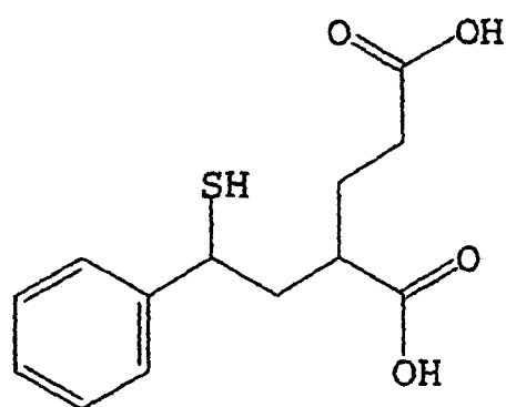
2-(2-phenyl-2-sulfanylethyl)pentanedioic acid
