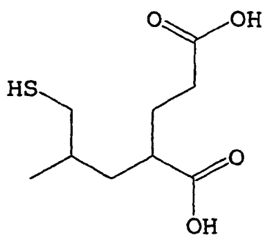
2-(3-sulfanyl-2-methylpropyl)pentanedioic acid
