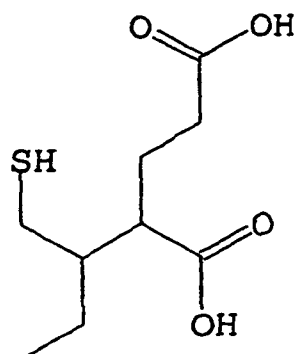
2-(1-ethyl-2-sulfanylethyl)pentanedioic acid
