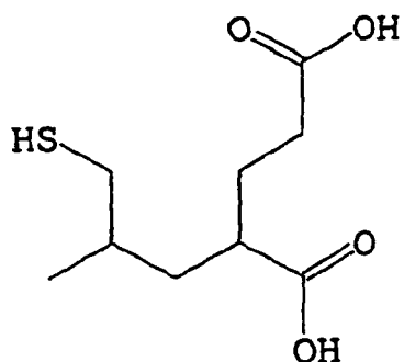
2-(3-sulfanyl-2-methylpropyl)pentanedioic acid
