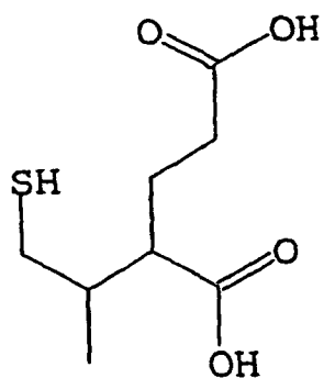
2-(1-methyl 2 sulfanylethyl)pentanedioic acid
