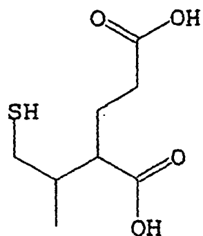
2-(1-methyl-2-sulfanylethyl)pentanedioic acid
