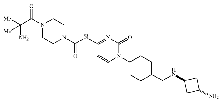
Diastereomer 2
