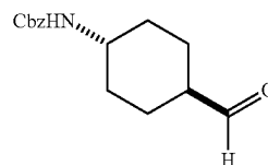
Benzyl (trans-4-formylcyclohexyl)carbamate
