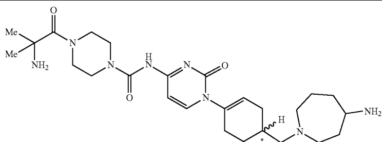
Diastereomer 2
