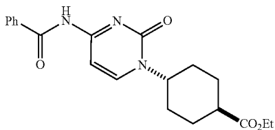
Ethyl trans-4-(4-benzamido-2-oxopyrimidin-1(2H)-yl)cyclohexane-1-carboxylate
