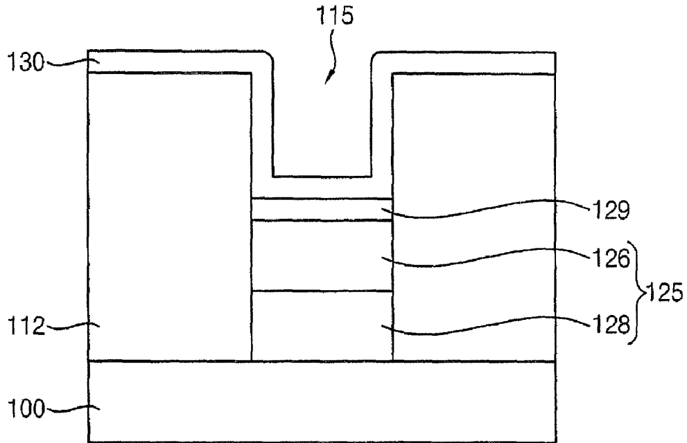
Figure 1C (Prior Art)
