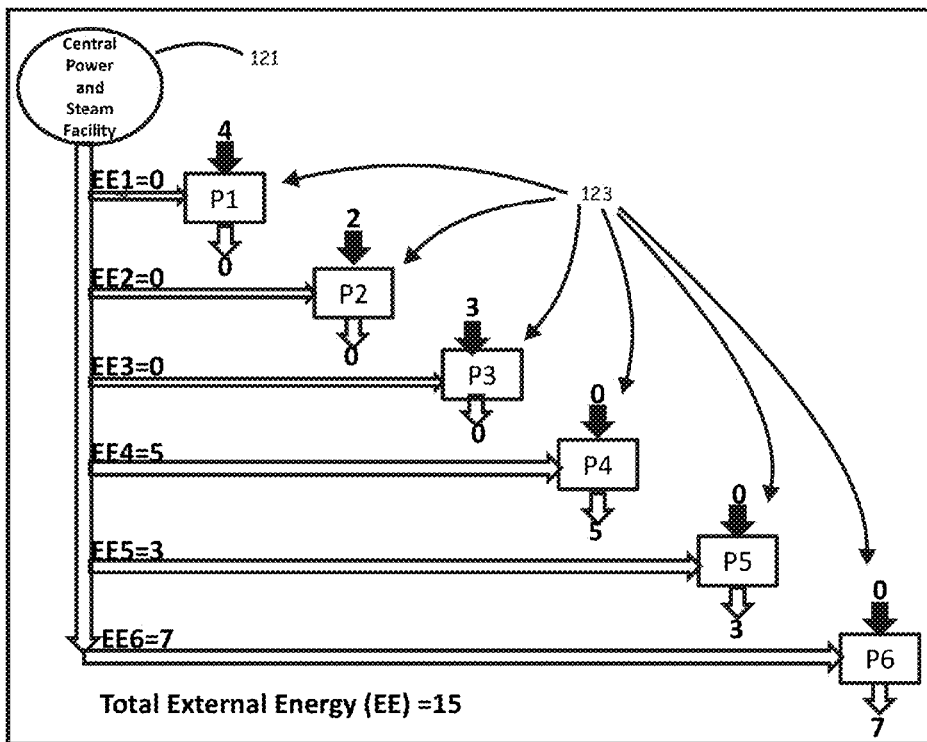
FIG. 22. (PRIOR ART)
