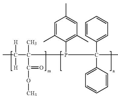
Co-polymer of 2-ethylhexylacrylate and phosphalkene
