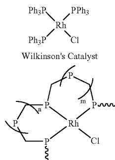
Polymer Supported Wilkinson's Catalyst n, m are greater than or equal to zero. Also, the coordinated phosphine groups may not all belong to the same polymer chain
