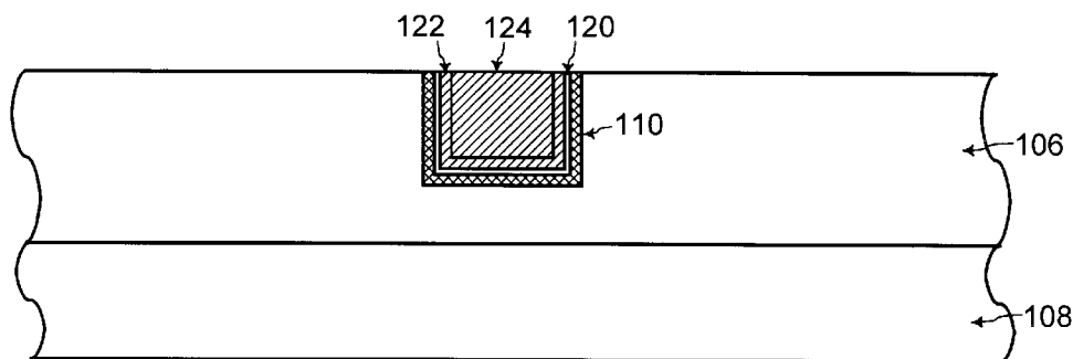
FIG. 5 (Prior Art)
