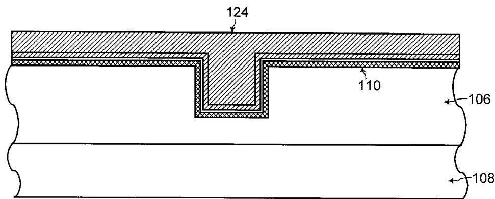
FIG. 4 (Prior Art)
