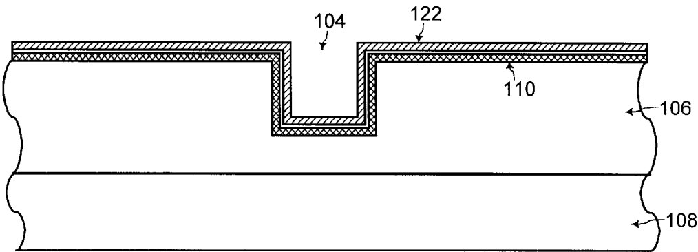
FIG. 3 (Prior Art)
