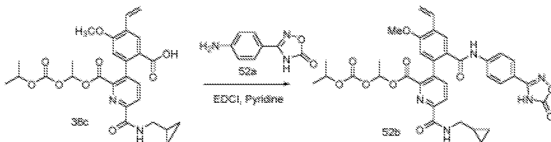
Scheme 52
