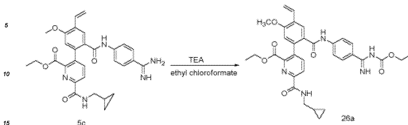
Scheme 26
