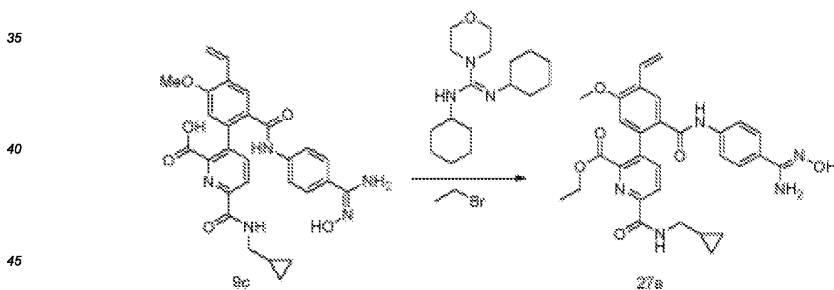
Scheme 27
