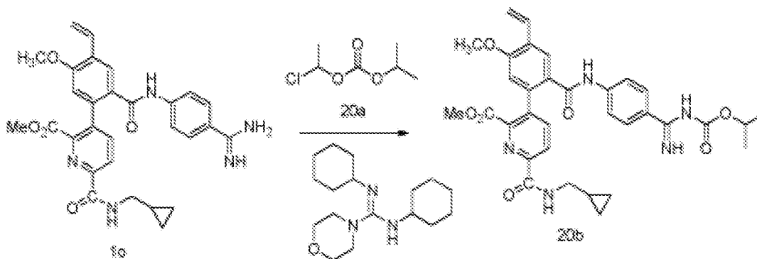
Scheme 20
