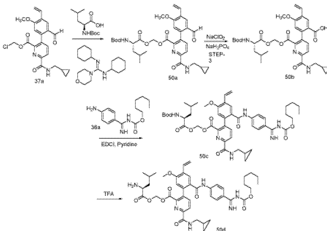
Scheme 50
