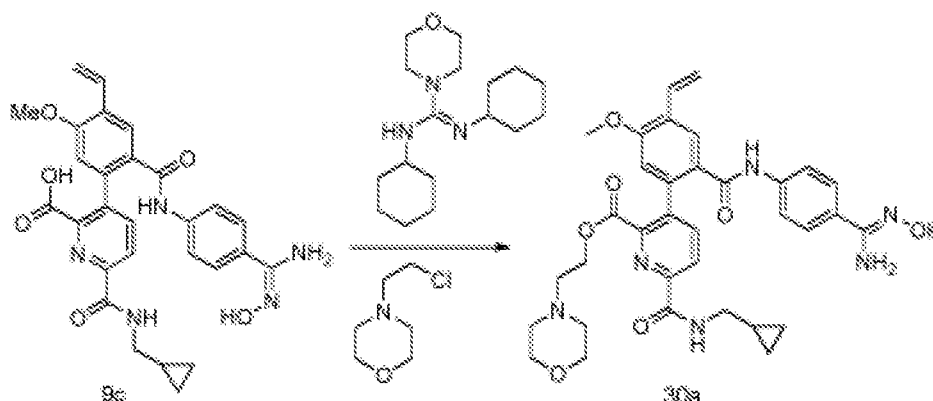
Scheme 30
