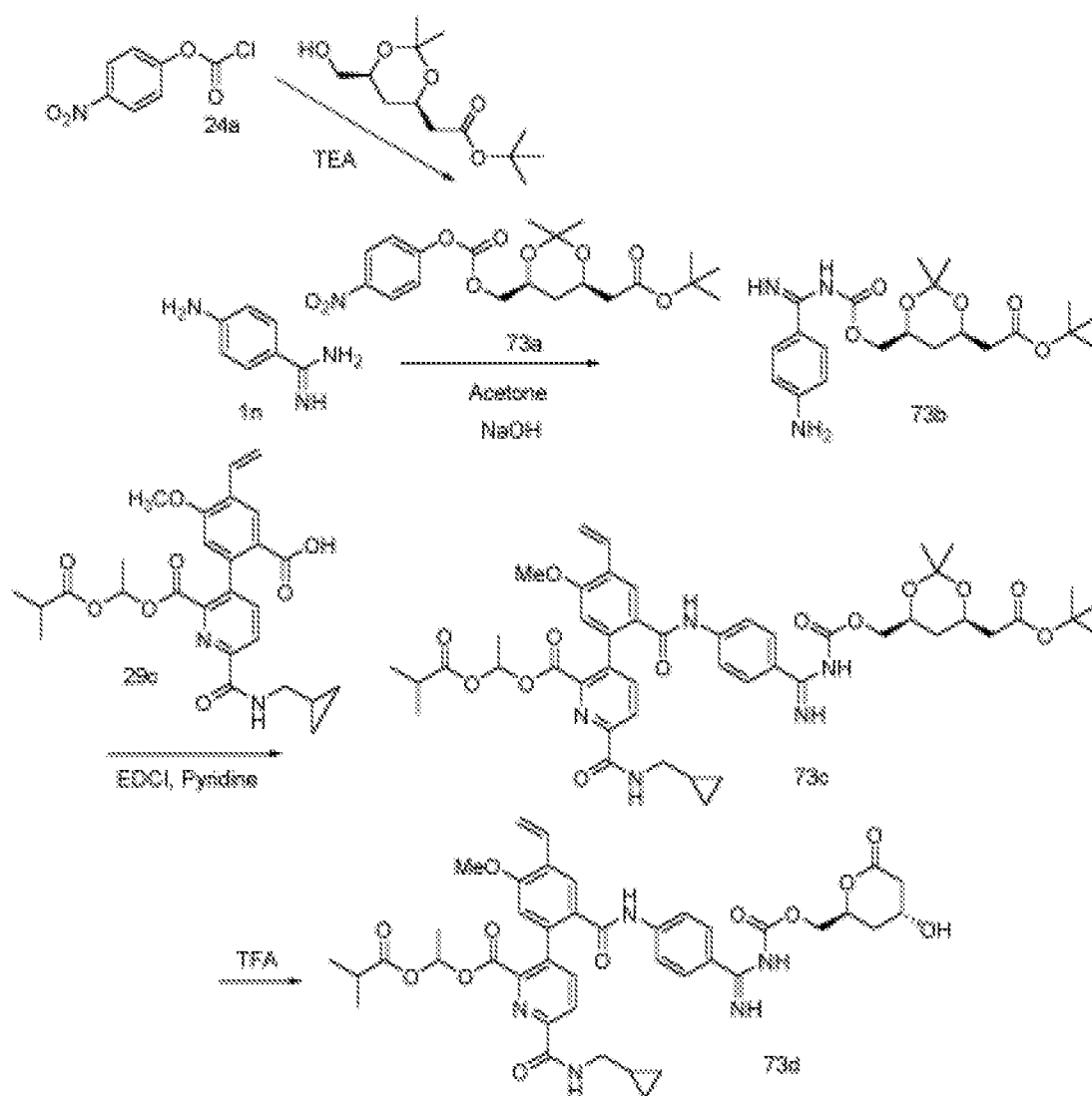
Scheme 73
