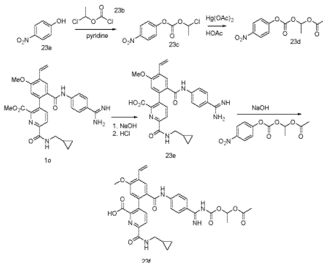
Scheme 23
