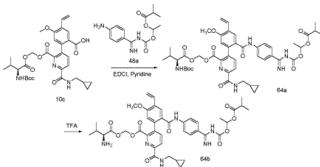
Scheme 64
