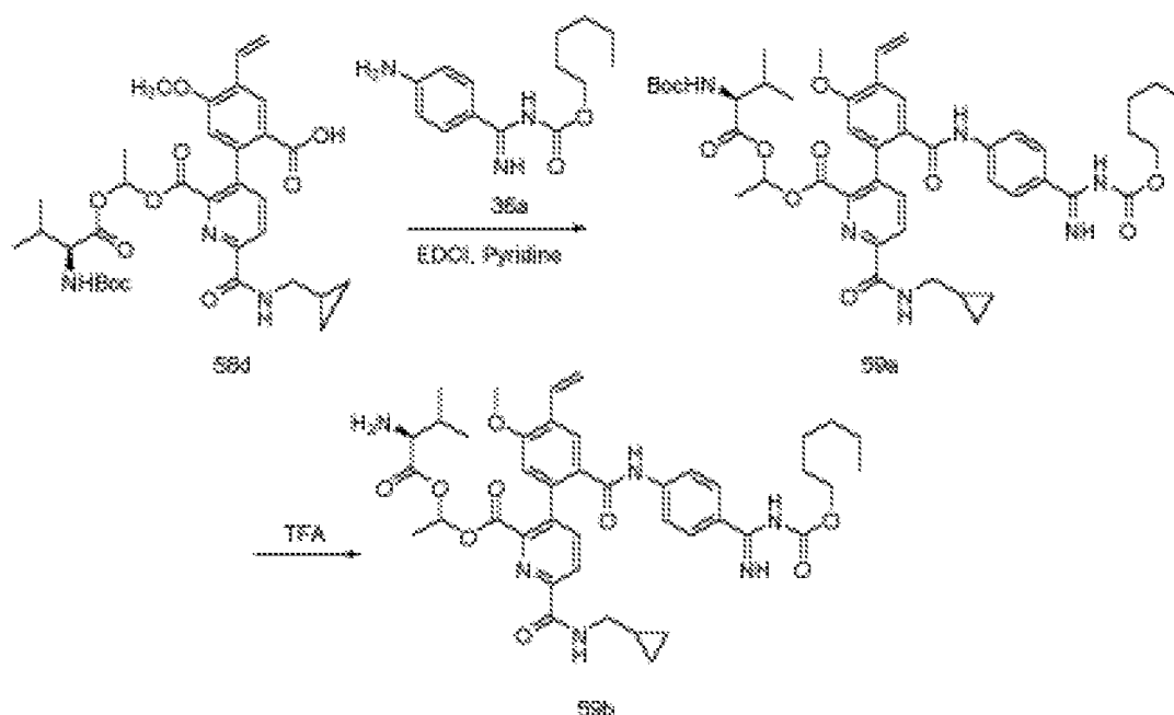
Scheme 59
