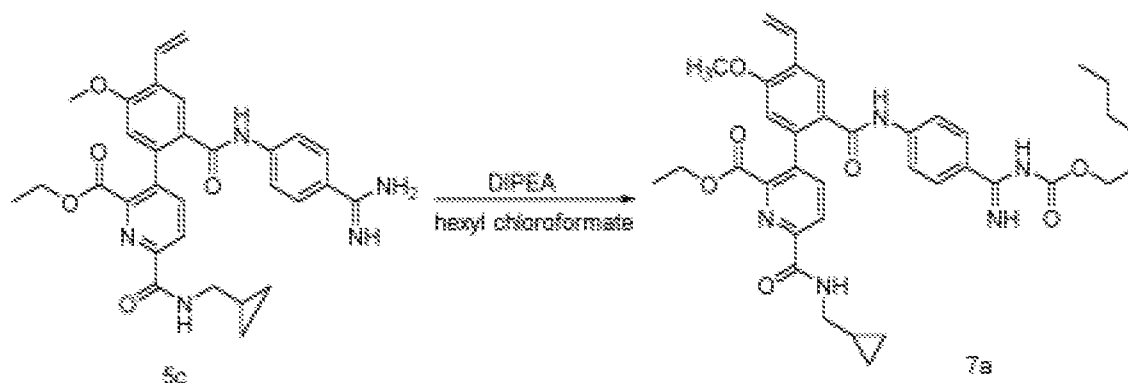
Scheme 7
