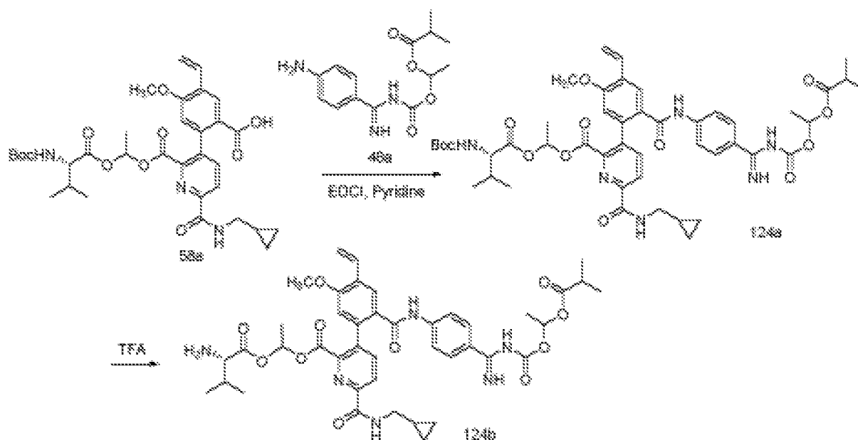
Scheme 124
