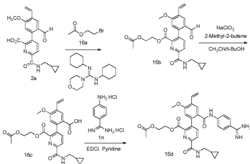
Scheme 16
