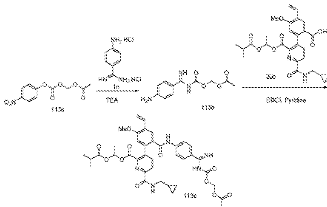
Scheme 113
