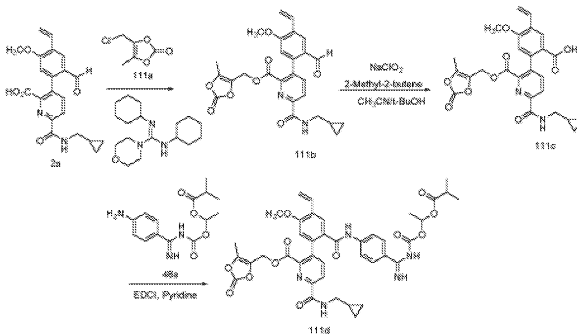
Scheme 111
