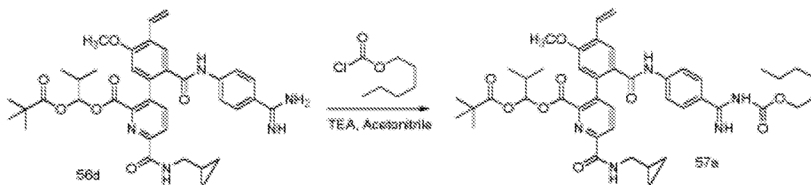
Scheme 57
