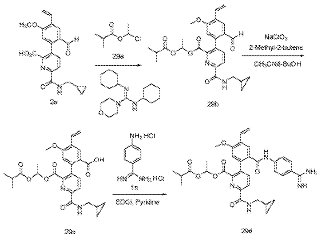
Scheme 29
