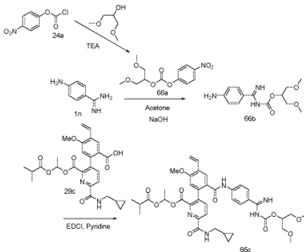
Scheme 66
