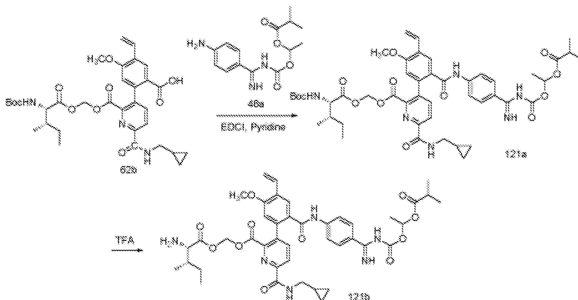
Scheme 121
