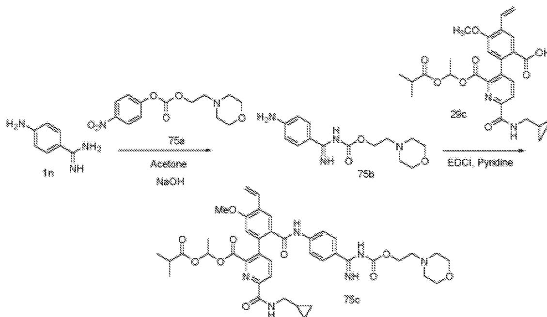
Scheme 75
