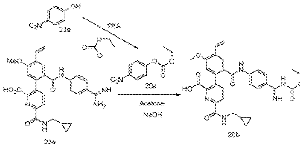
Scheme 28
