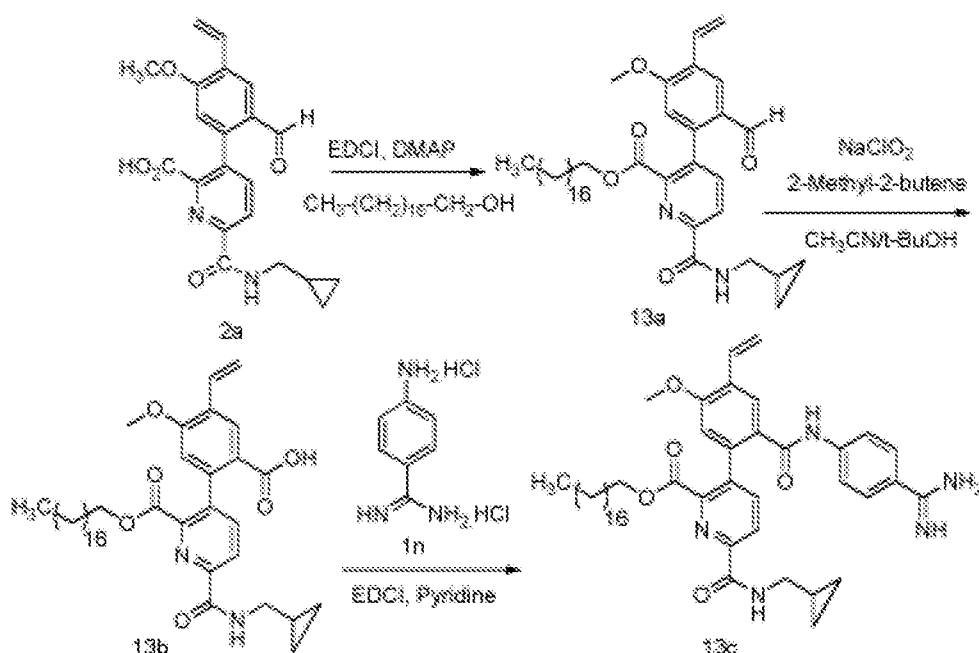
Scheme 13
