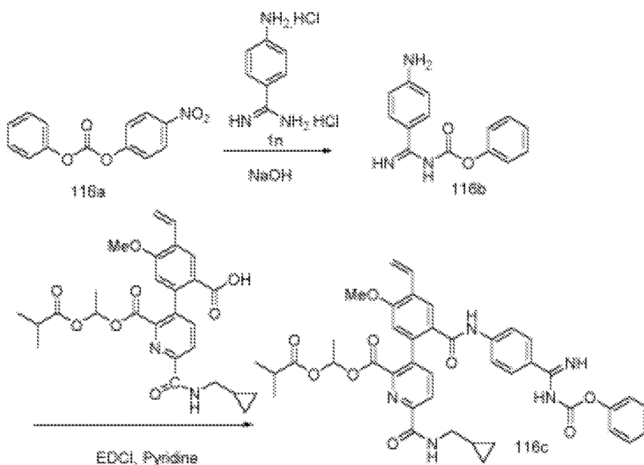
Scheme 116
