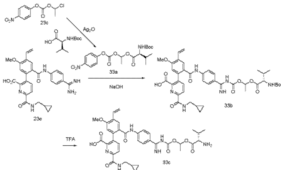
Scheme 33
