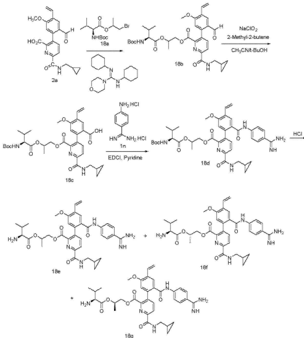
Scheme 18
