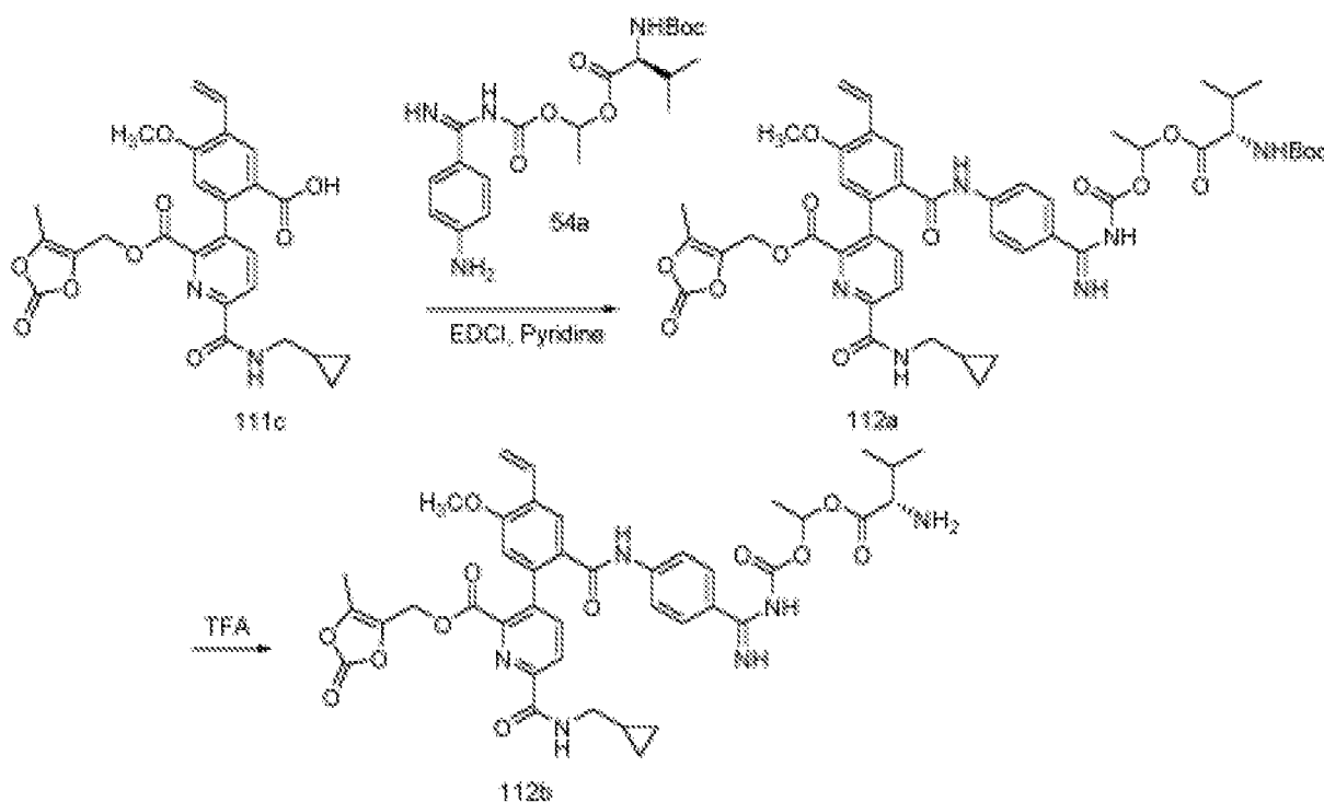
Scheme 112
