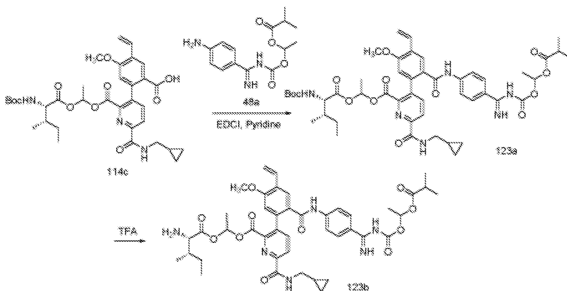
Scheme 123
