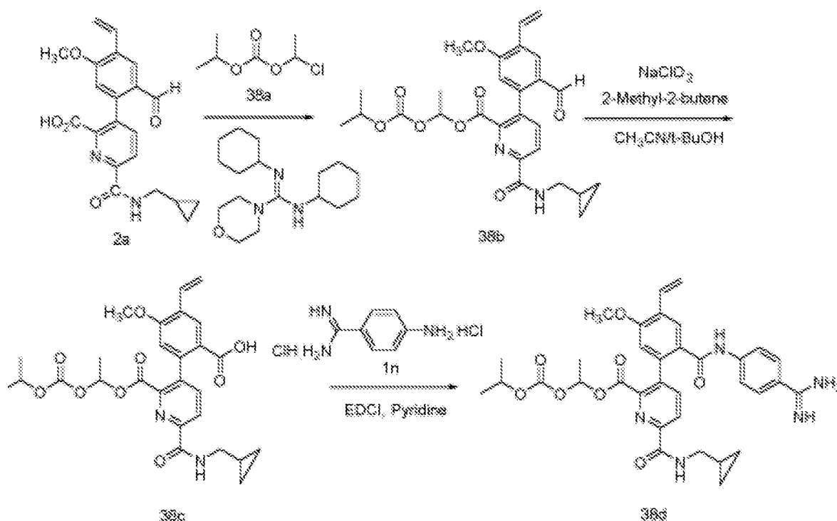
Scheme 38
