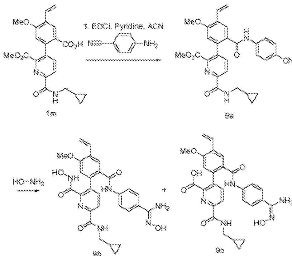
Scheme 9
