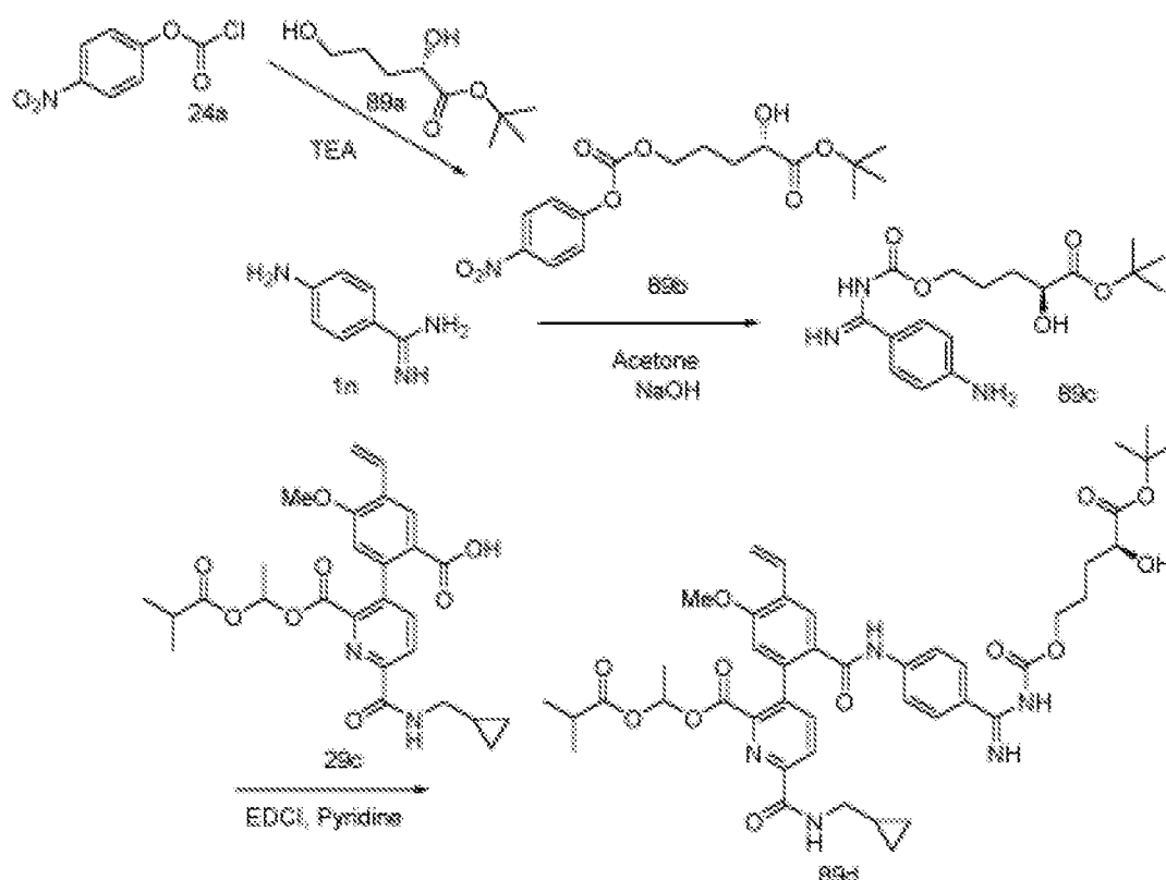
Scheme 89
