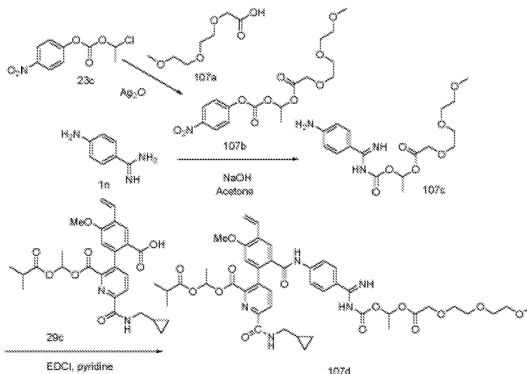
Scheme 107
