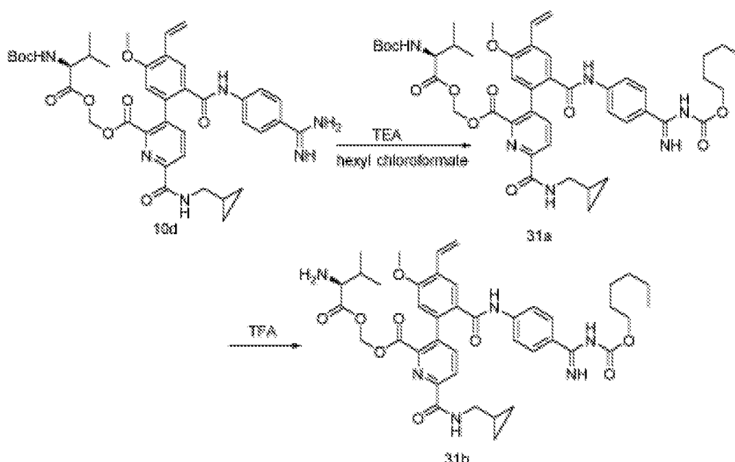
Scheme 31
