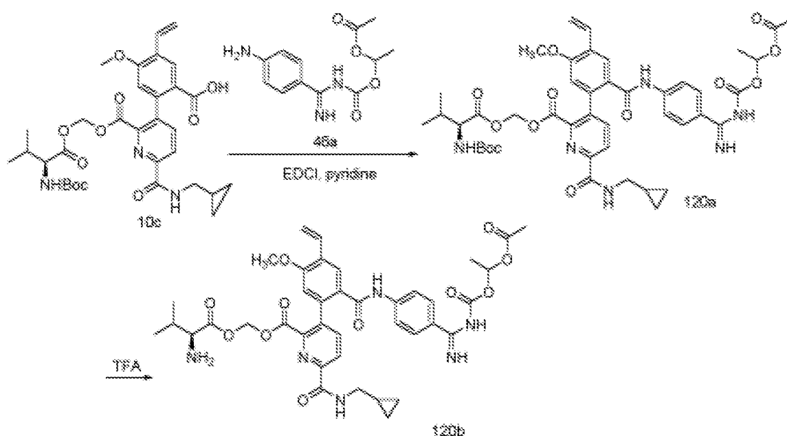
Scheme 120
