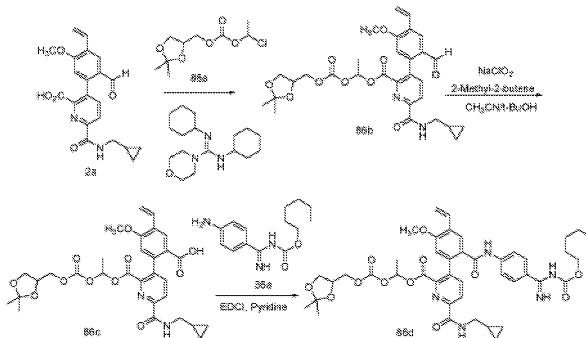
Scheme 86
