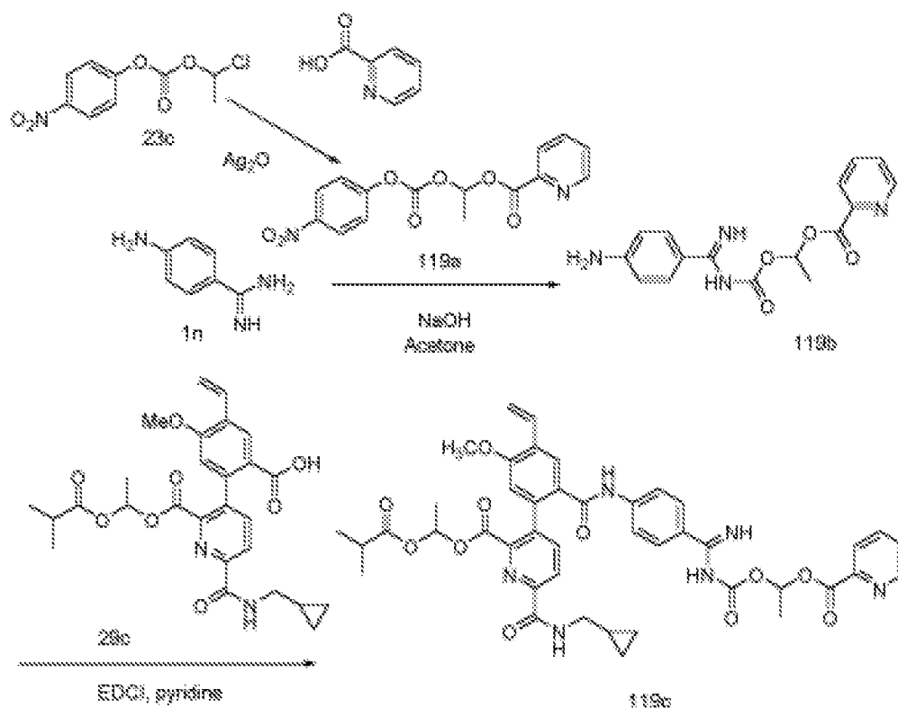
Scheme 119
