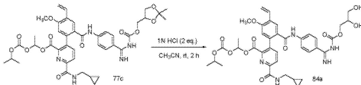
Scheme 84
