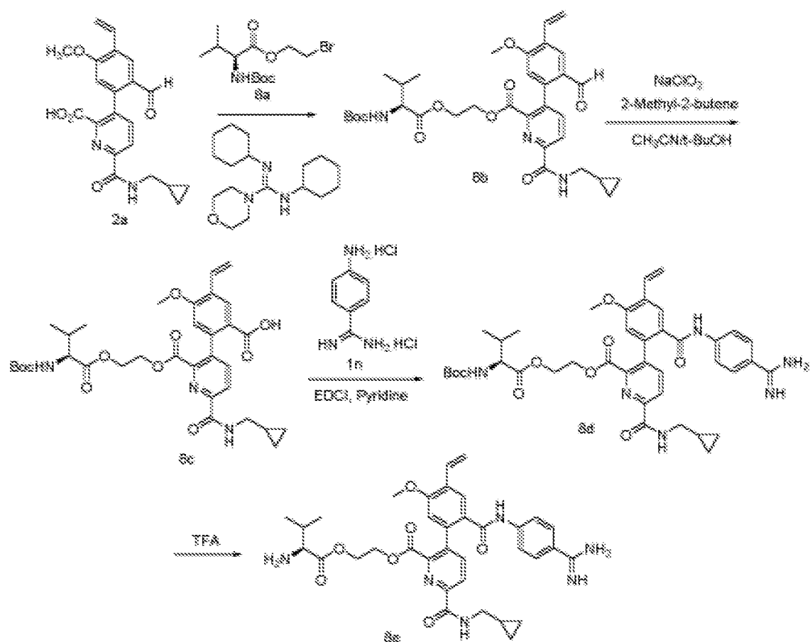
Scheme 8
