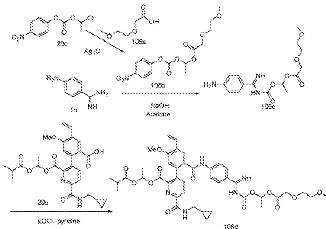
Scheme 106
