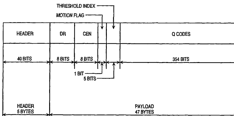
PACKET STRUCTURE 300
