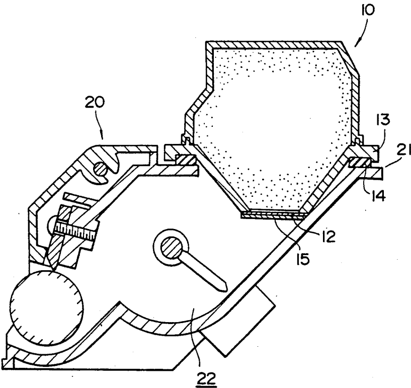
FIG. 4 PRIOR ART
