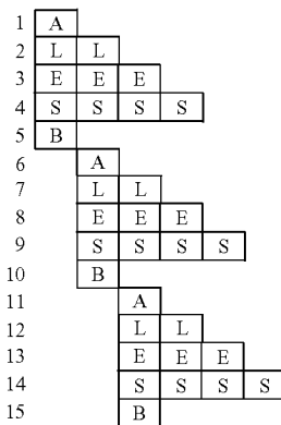
Superstring pipeline
