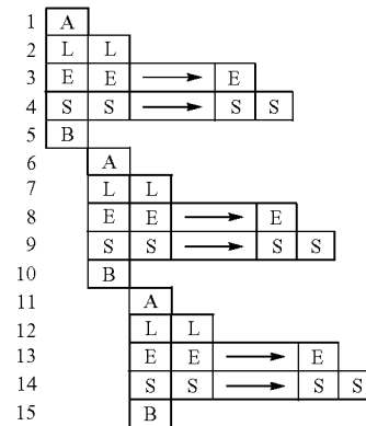
Superspring pipeline
