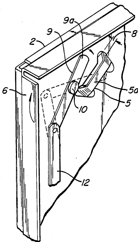
FIG. 7. PRIOR ART
