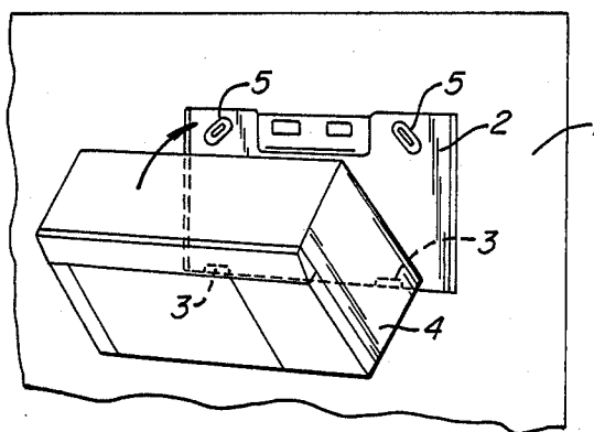
FIG. 5. PRIOR ART
