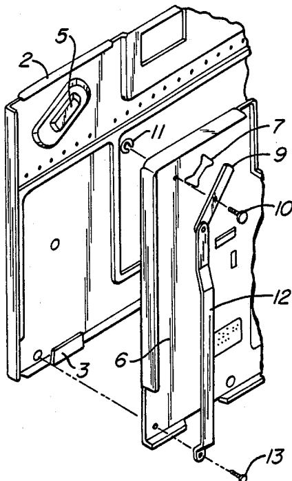
FIG. 6. PRIOR ART
