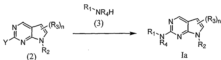
Reaction Scheme I
