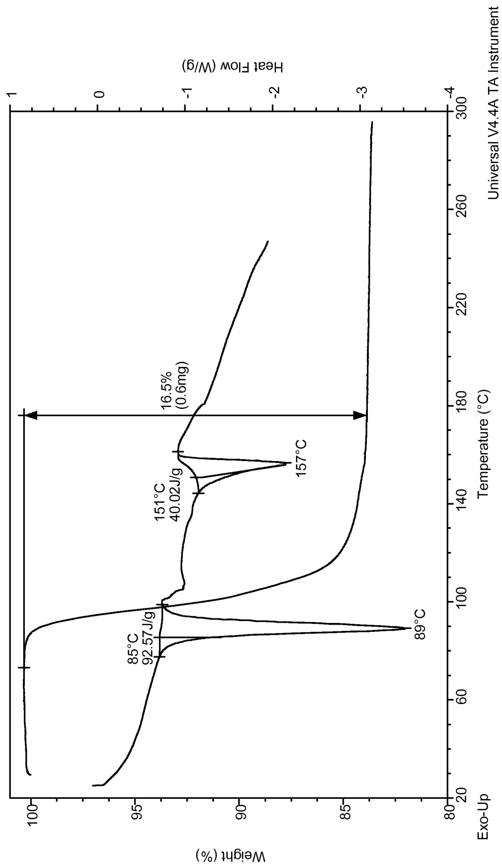
FIG. 15 TGA/DSC Thermograms of Form E
