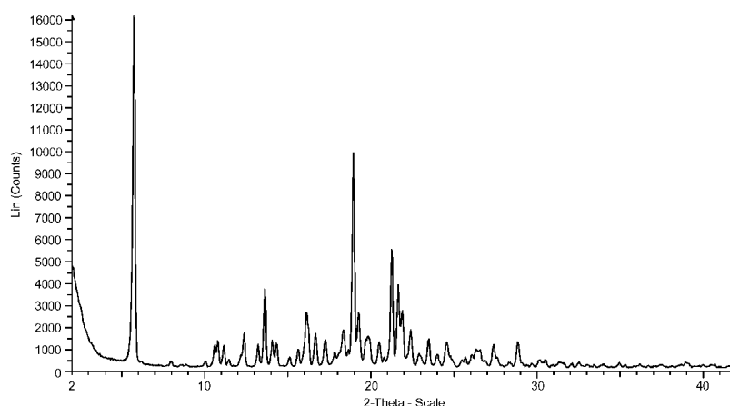
FIG. 1 XRPD Pattern of Form A
