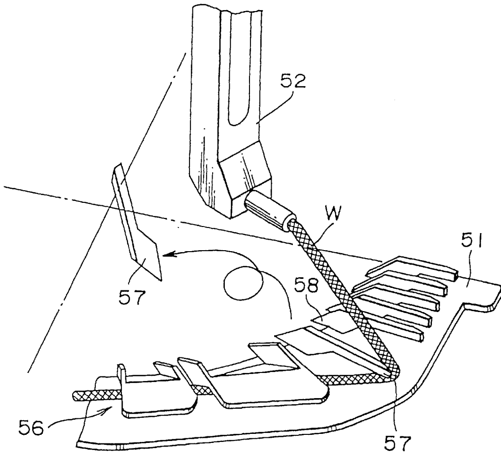
FIG. 4 (PRIOR ART)
