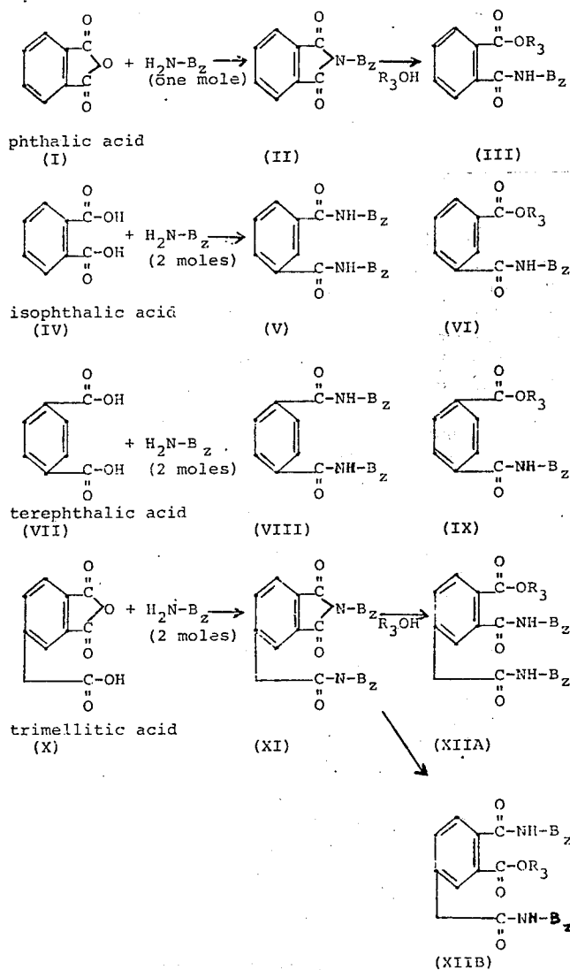
FLOW SHEET I
