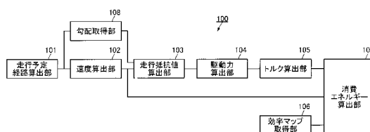
Fig. 1 101 Scheduled travel route calculating unit 102 Speed calculating unit 103 Travel resistance value calculating unit 104 Driving force calculating unit 105 Torque calculating unit 106 Efficiency map acquiring unit 107 Energy consumption calculating unit 108 Gradient acquiring unit
