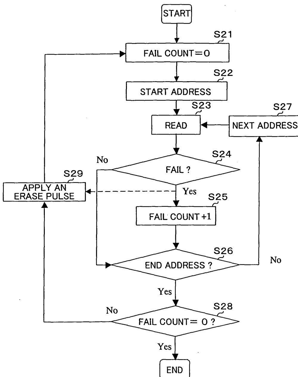
FIG. 4 (PRIOR ART) ERASE VERIFICATION
