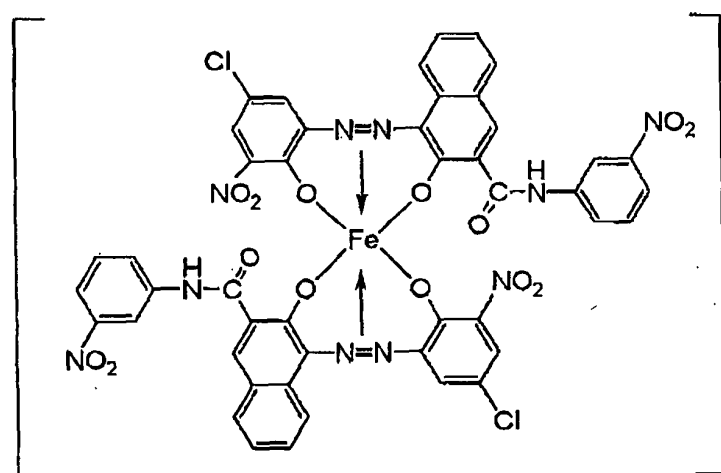
azo type iron complex compound (4)
