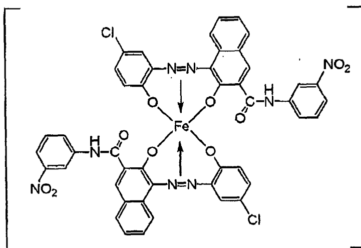
azo type iron complex compound (4)
