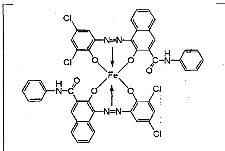
azo type iron complex compound (3)
