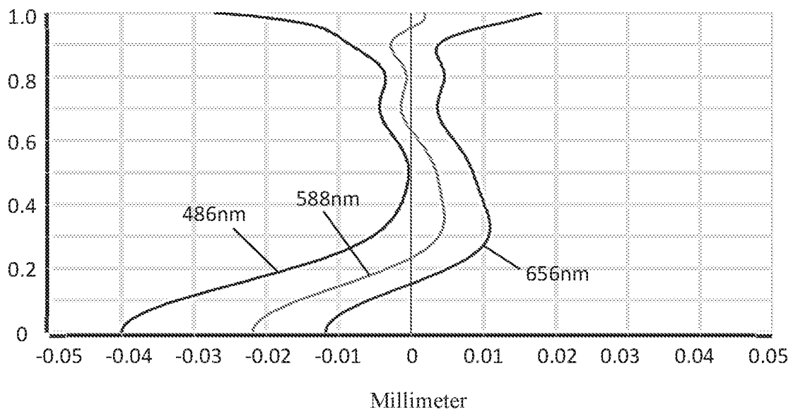
Longitudinal Aberration
