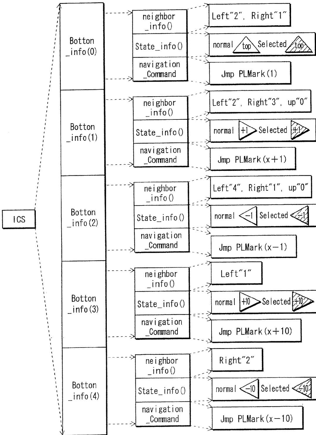
DATA STRUCTURE OF ICS (PTS=tx)
