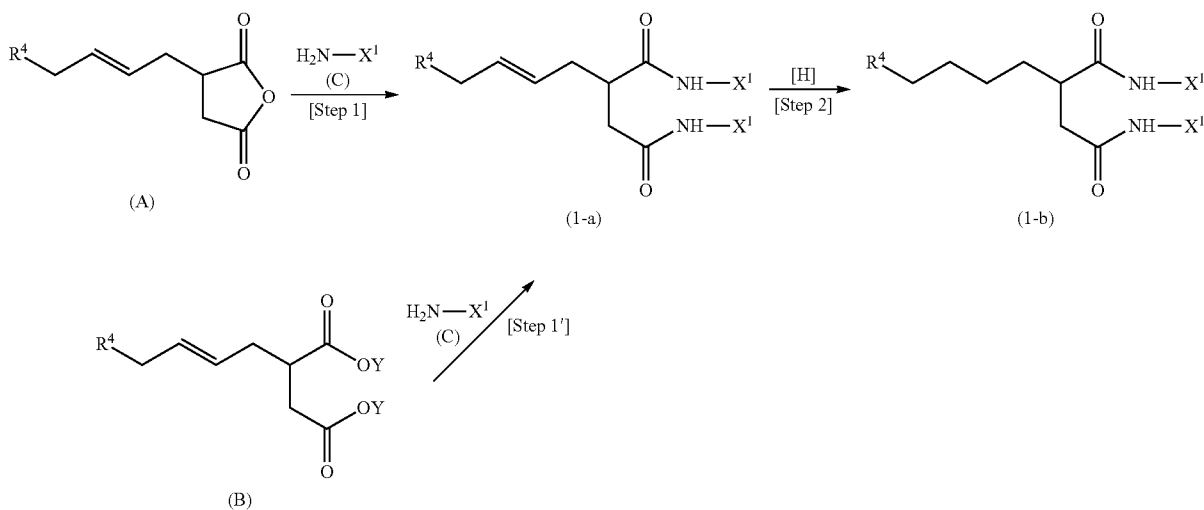
<Reaction 1>
