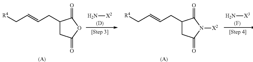
<Reaction 2>
