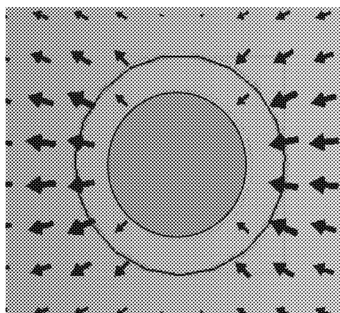
Conductor mode (HE11) 2057
