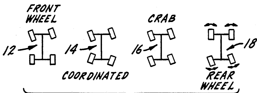
FIG. 1. ( STEERING MODES )
