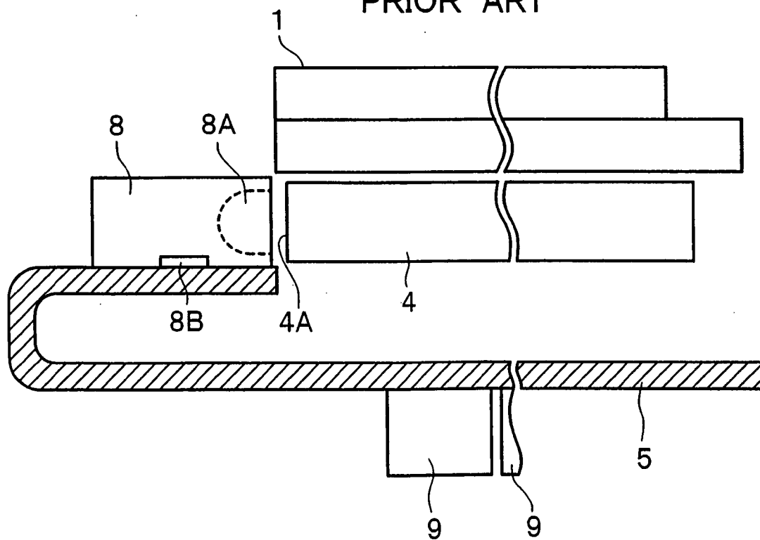
FIG. 15 PRIOR ART
