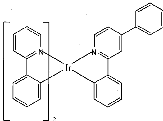
Compound 1
