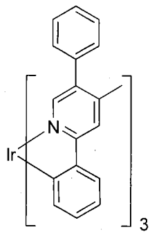
Compound 21
