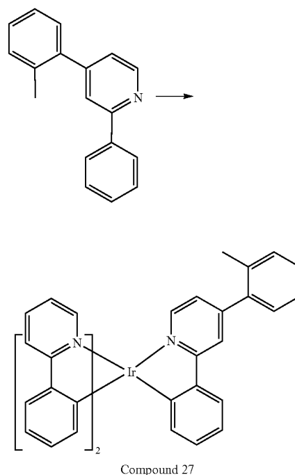
Compound 27
