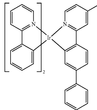
Compound 9
