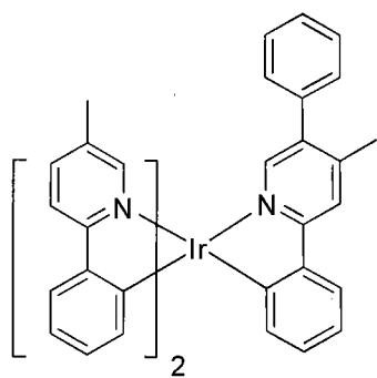
Compound 31
