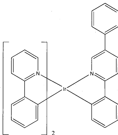
Compound 2
