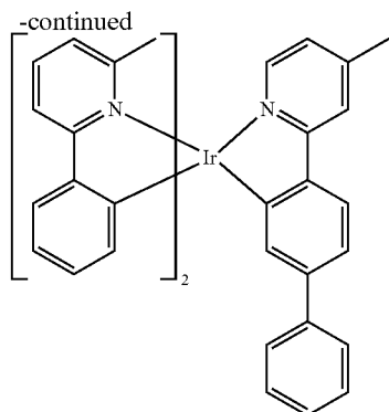
Compound 10
