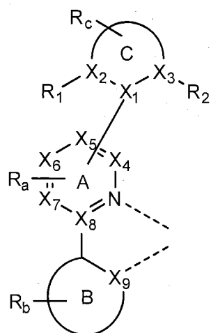
Formula I
