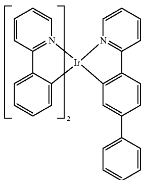
Compound 8
