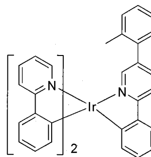
Compound 25
