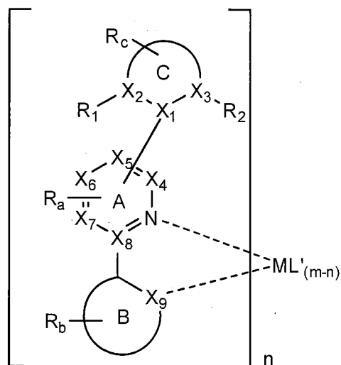
Formula II
