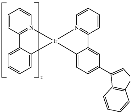
Compound 2
