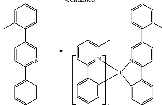
Compound 26
