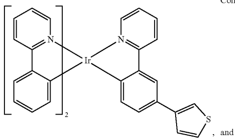
Compound 5
