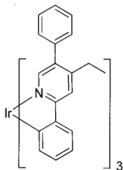
Compound 22
