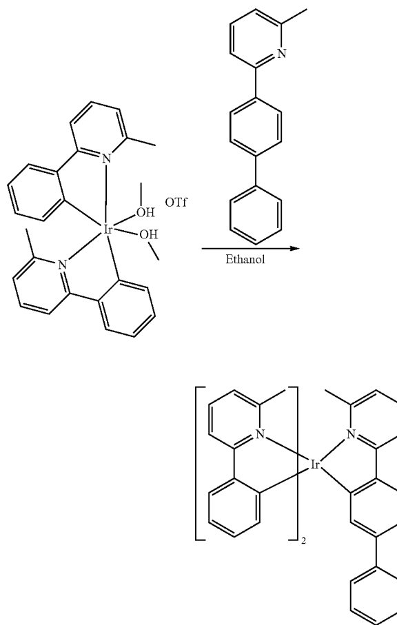
Compound 13
