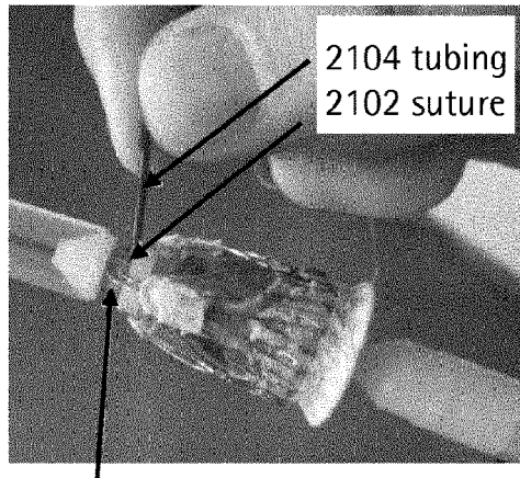
2106 stentholder with pins
