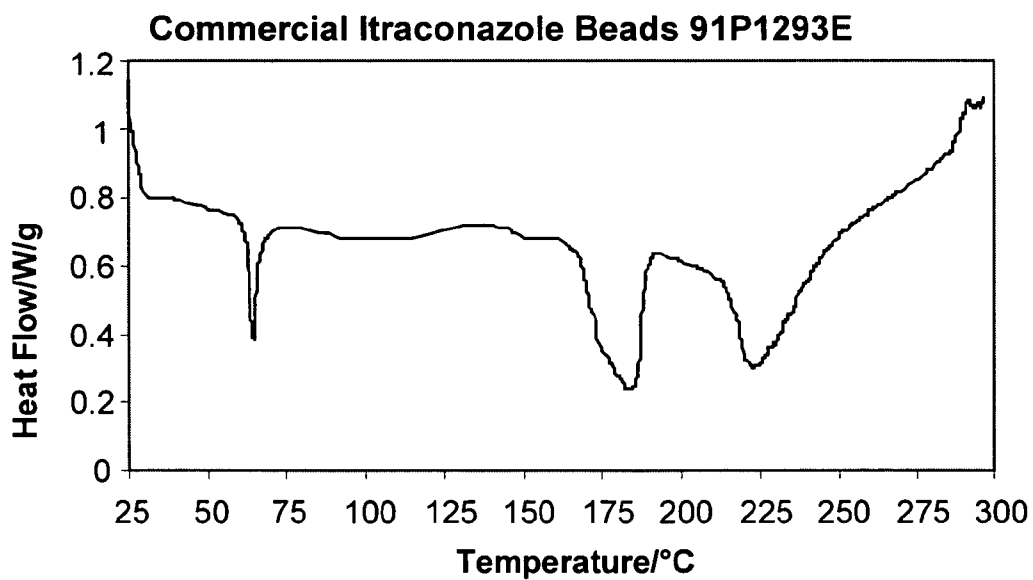
Figure 4: Normalized DSC thermogram of commercially available itraconazole loaded beads
