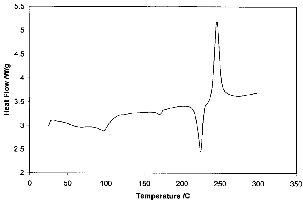
Figure 9: Normalized thermogram of Paclitaxel Active Pharmaceutical Ingredient
