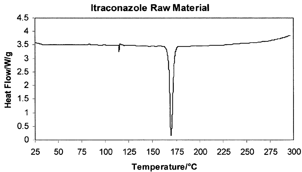
Figure 2: Normalized DSC thermogram for Itraconazole activepharmaceutical ingredient
