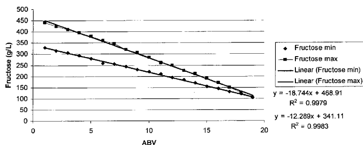
Fig. 1. Fructose v ABV (9 Celsius degree window)
