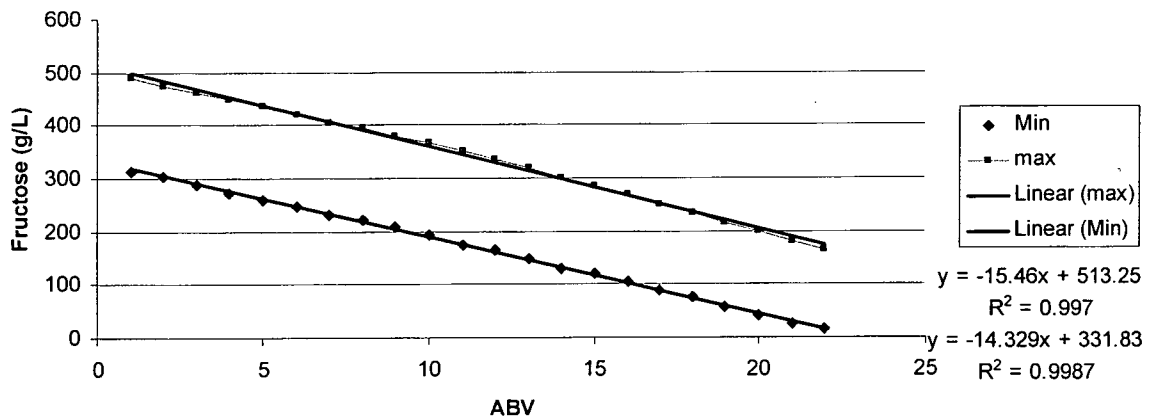
Fig. 2. Fructose v ABV (5 Celsius degree window)
