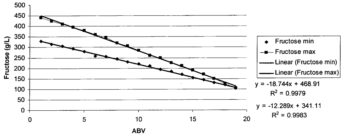
Fig. 1. Fructose v ABV (9 Celsius degree window)
