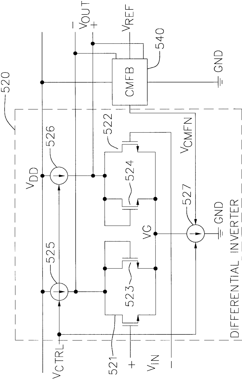
410 FIG. 5 DIFFERENTIAL DELAY CIRCUIT
